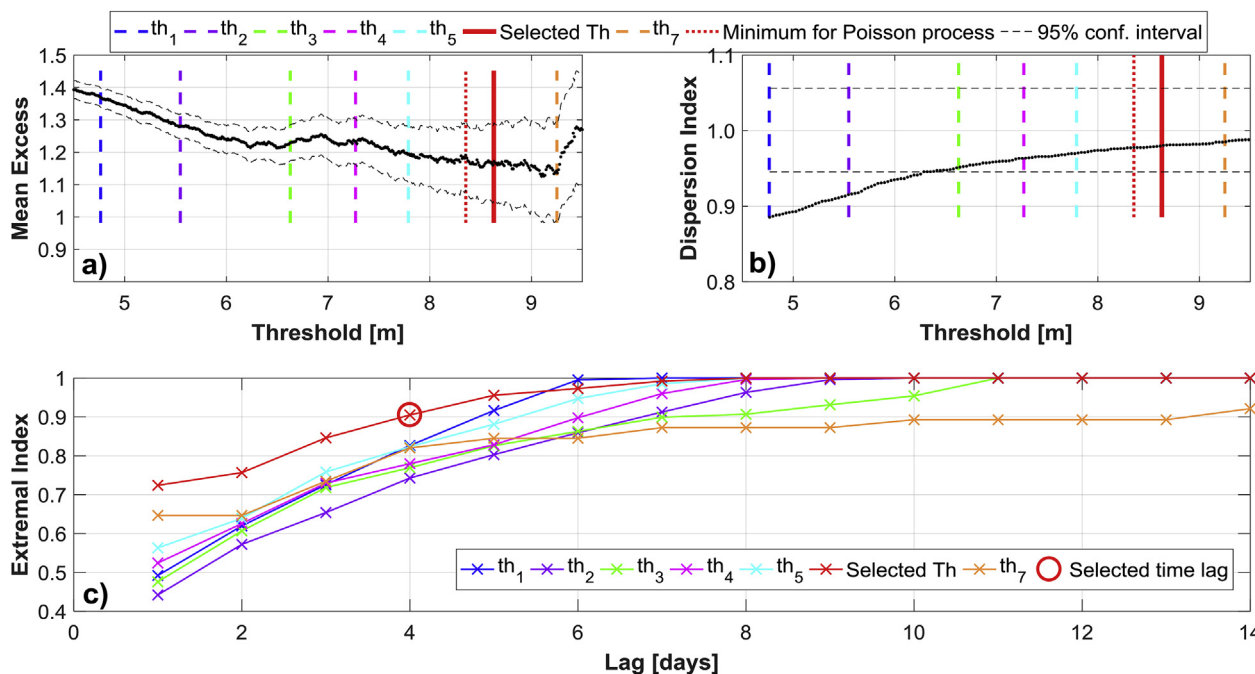
Fig. 5. a), mean residual life plot, 95% confidence intervals based on the approximate normality of sample means, b) dispersion index considering all 7 investigated thresholds and c) extremal index for combination of all seven investigated thresholds and 14 declustering time lags.
