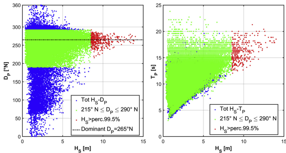
Fig. 3. Fastnet offshore wave climate.
