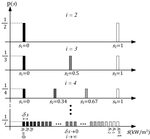
Fig. 2. Probability distributions p(s) of PV module shading problem for different number of irradiance levels i . \delta s is the difference value between two consecutive irradiance levels.
