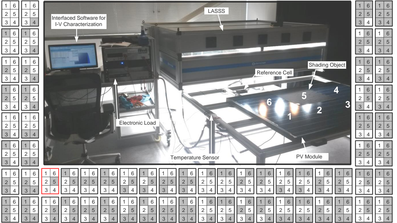
Fig. 3. Indoor experimental setup for testing shading tolerability along with 64 shading profile codes from 000000 to 111111. The depicted module under test (#4, see Table I) has 54 cells and is divided into 6 sections. The 010000 shading profile code is shown in the figure. In the figure, sections 1, 2, 3, 4, and 6 are about to receive rated irradiation ( 1000 \text{ W/m}^2 ) while section 5 is shaded and receives 250 \text{ W/m}^2 . The shading object for this specific module shades simultaneously 9 cells.
