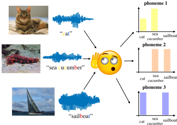
Figure 1: Illustration of semantic-driven phoneme discovery
