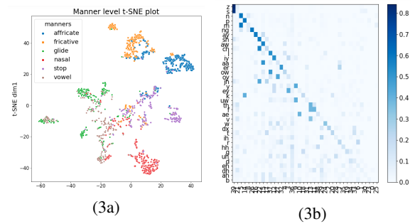
Figure 3: Left: Manner-level t-SNE plot by IQ with |\mathbb{Y}| = 824 and gold segmentation on TIMIT. Right: Distribution of codeword assignment for each phoneme by IQ with |\mathbb{Y}| = 824 and predicted segmentation on TIMIT. Each row of the plot is the empirical distribution for P_{\hat{z}|Z}(\cdot|z) , 1 \leq z \leq K , where the phonemes are sorted top-to-bottom with decreasing \max_{z'} P_{\hat{z}|Z}(z'|z) .
