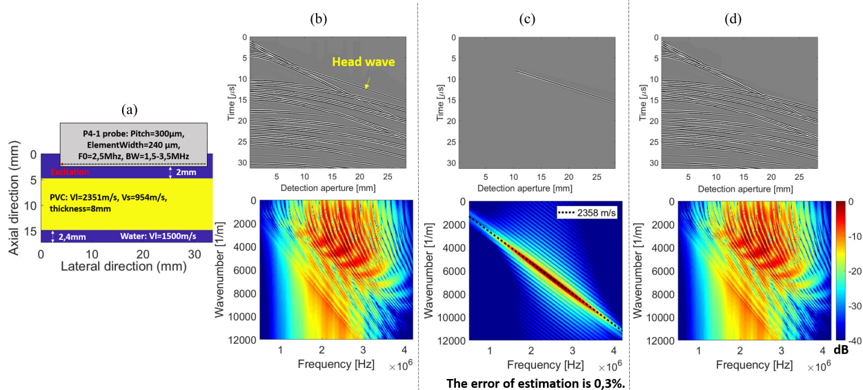
Fig. 1. (a) Numerical model used in SimSonic. F_0 , BW , V_L , and V_s are the central frequency, bandwidth, longitudinal wave velocity, and transverse wave velocity, respectively. (b)–(d) Numerical space–time domain data and the corresponding f-k representation. (b) All the data. (c) Only the head wave. (d) Head wave is removed.
