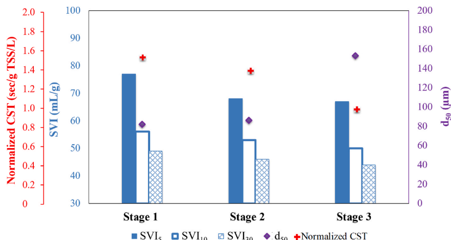
Fig. 3. SVI, d_{50} , and normalized CST values of the sludge in AGS process.
