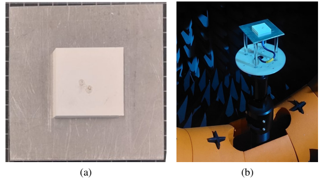
Fig. 5. (a) Finished 3D printed stacked patch antenna for GNSS applications mounted on an aluminum ground plane. (b) Mounting of the antenna in an MVG Starlab anechoic chamber.
