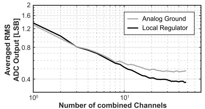
Fig. 19. Investigation of the noise output of the array as a function of the number of combined channels with the LNAs being connected to the shared analog ground or local negative supply regulators.
