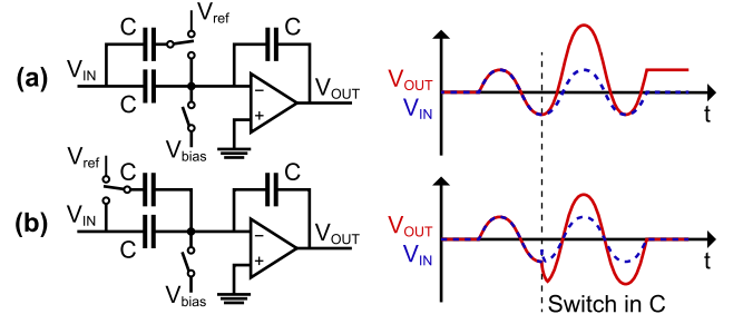
Fig. 9. Impact of switching the gain of an amplifier in a dynamically biased capacitive feedback in active operation from (a) back and (b) front.
