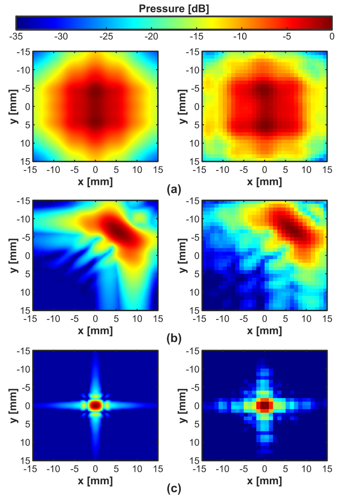
Fig. 18. Comparison of simulated C -planes on the left and corresponding measured C -planes on the right for (a) diverging beam at 5 cm from the array, (b) plane wave steered to the northeast at 5 cm from the array, and (c) focused beam at 2 cm from the array.
