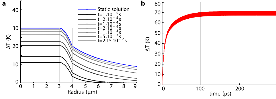
FIG. 9. (Color online) (a) Convergence of the FDM simulation result towards the static solution. This simulation is performed for a 3\mu\text{m} radius bubble with a 1\mu\text{m} thick triacetin oil layer and a continuous laser exposure and (b) simulation result of the same bubble irradiated with a laser intensity modulated at 1 MHz, showing the quasi-convergence of the gas temperature after 100\mu\text{s} .
