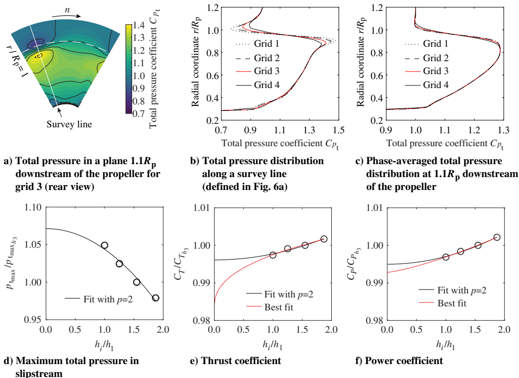
Fig. 6 Mesh refinement study for the isolated propeller grids.
