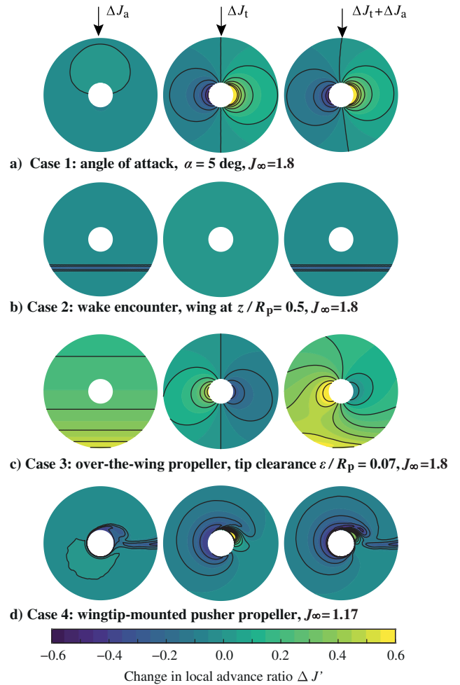
Fig. 11 Computed inflow profiles of the four validation cases that are used as input to the method.
