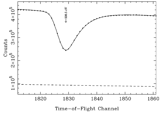
FIG. 3. Sample fit to time-of-flight (TOF) spectrum for the resonance at 500.5 eV. The counts are for one run and are summed over the two helicity states. The dashed line is the background.
