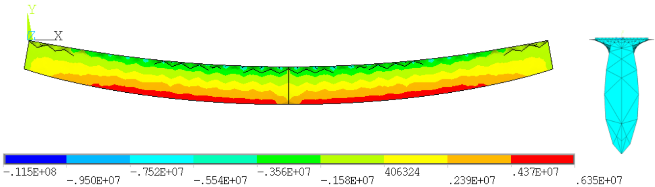
Figure 8.17 Front view and cross-section of the optimized beam at generation from Run 33, subjected to loading. Resulting stresses in x-direction are in [N/m 2 ]
