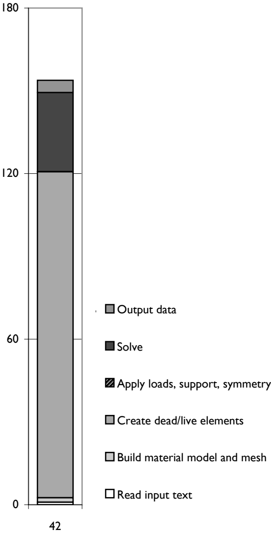
Figure 7.10 Diagram showing the computational demand of the ANSYS analysis in seconds for a solution in FABRICFORMER.
