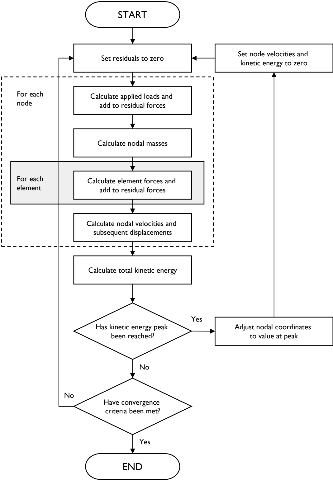
Figure 5.5 Flowchart describing the BESO algorithm
