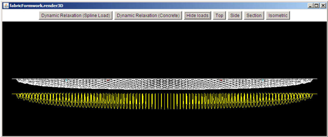
Figure 7.6 Early screenshot of the FABRICFORMER GUI including visualization of the concrete pressures.
