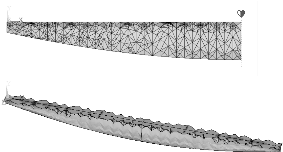
Figure 6.18 Example of a free meshed fabric formed beam. The x-coordinates of the nodes have been averaged result- ing in parallel slices in the yz-plane, prior to meshing.
