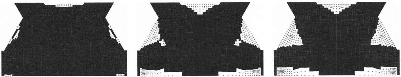
Figure 2.4 This particular thesis focused on creating a least-weight topology for large steel nodes. Such nodes are cast to avoid welds in critical high stress areas and reduce the chance of fatigue failure. They can be found in large steel structures, such as offshore platforms.
