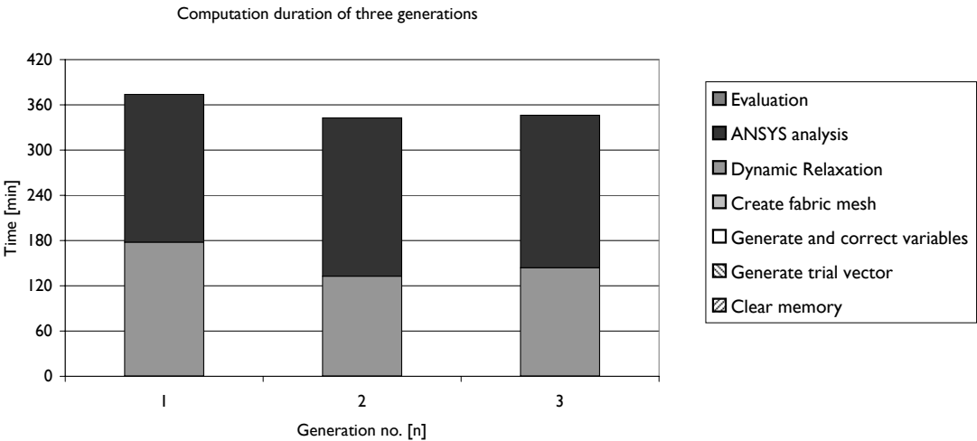
Figure 7.7 Diagram showing the computational demand in minutes for three generations in FABRICFORMER each calculating fifty beams.
