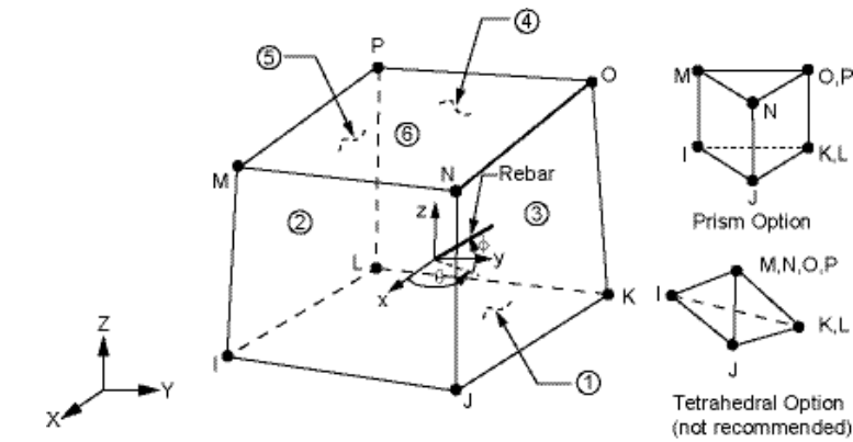
Figure 6.17 SOLID65 Element, also in prism and tetrahedral form. ANSYS 11.0 User Manual (2008).
