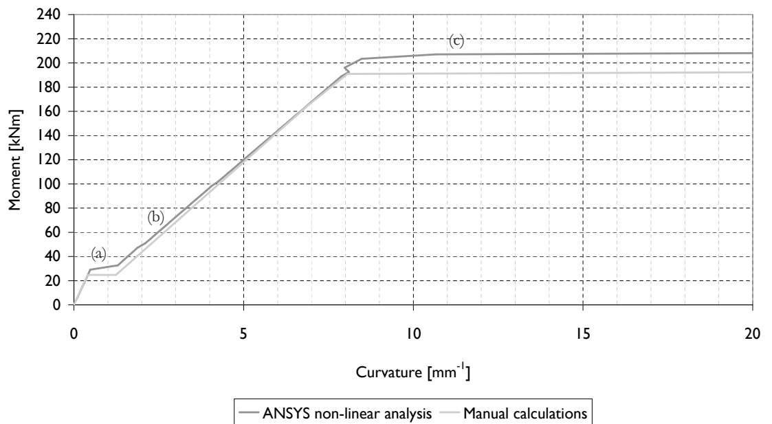
Moment-curvature diagram
