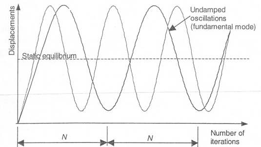
Figure 5.1 Undamped structural motion in time (Top left) Barnes (1998)
