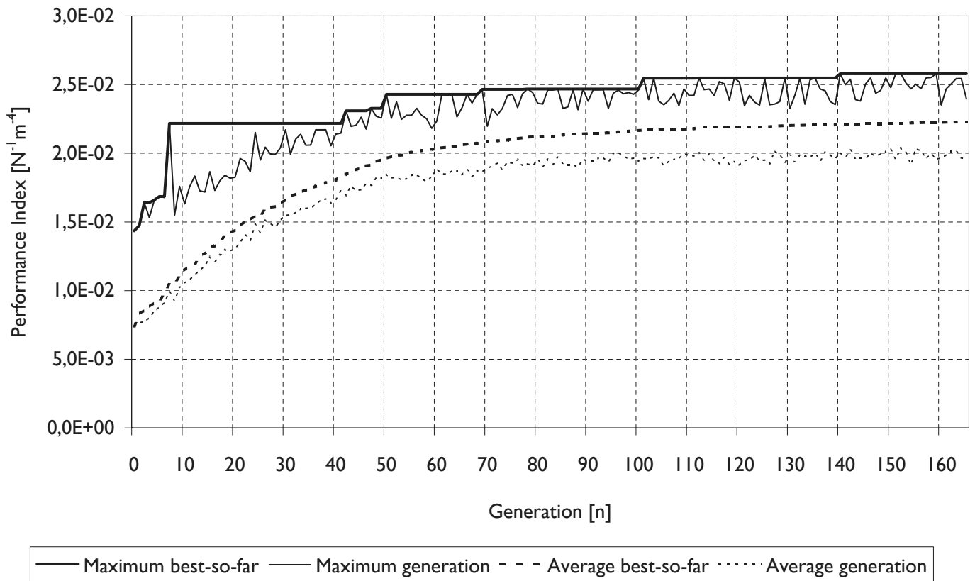
Performance Index for keel mold (Run no. 33)
