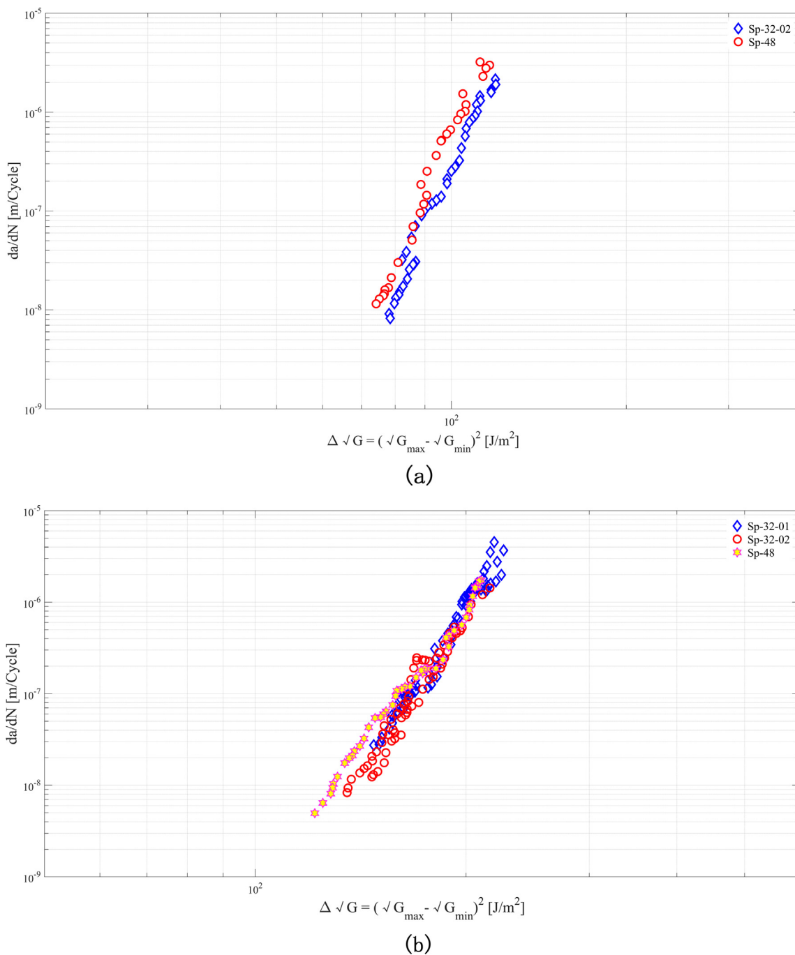
Fig. 9. The significance of fibre bridging in FDG (a) a-a_0 is around 20 mm; (b) Plateau state. (For interpretation of the references to colour in this figure legend, the reader is referred to the web version of this article.)
