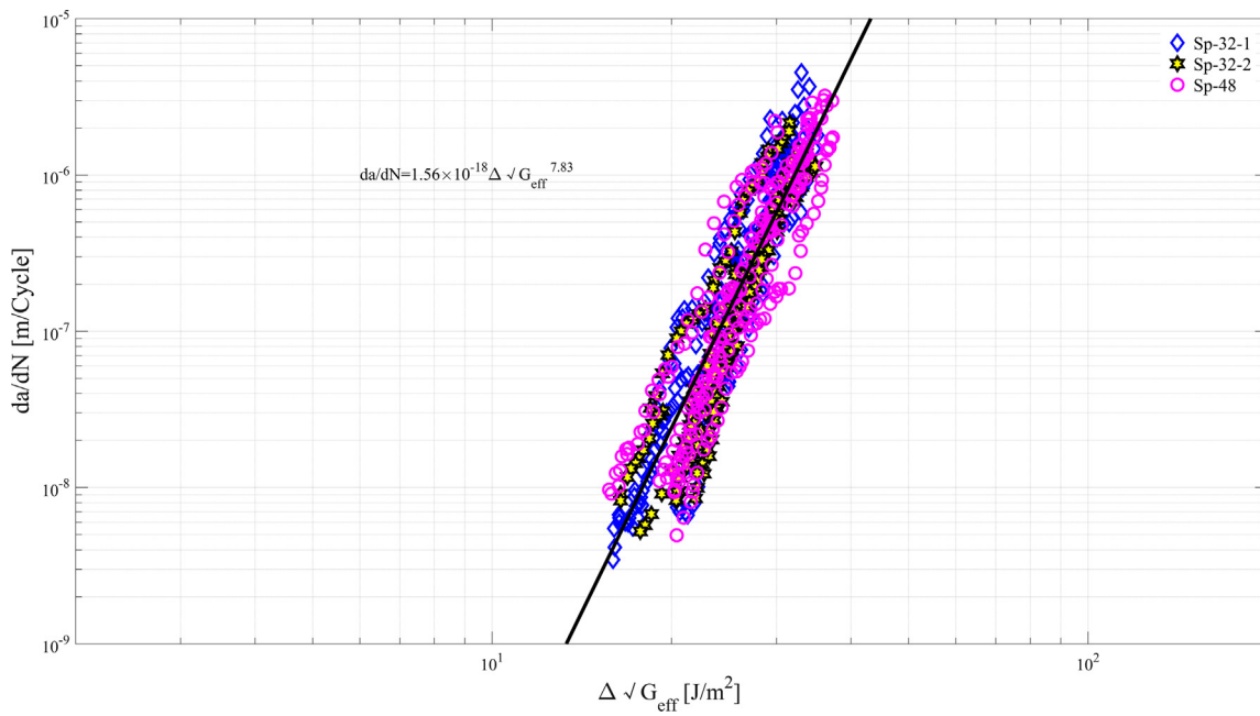
Fig. 12. Fibre-bridged fatigue delamination in multidirectional composite laminates. (For interpretation of the references to colour in this figure legend, the reader is referred to the web version of this article.)
