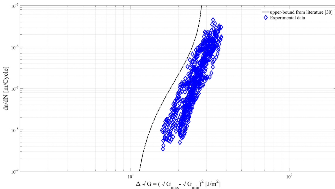
Fig. 13. A comparison between the upper bound FDG curve calculated via the methodology proposed in literature [30] and the experimental data interpreted via the modified Paris relation. (For interpretation of the references to colour in this figure legend, the reader is referred to the web version of this article.)
