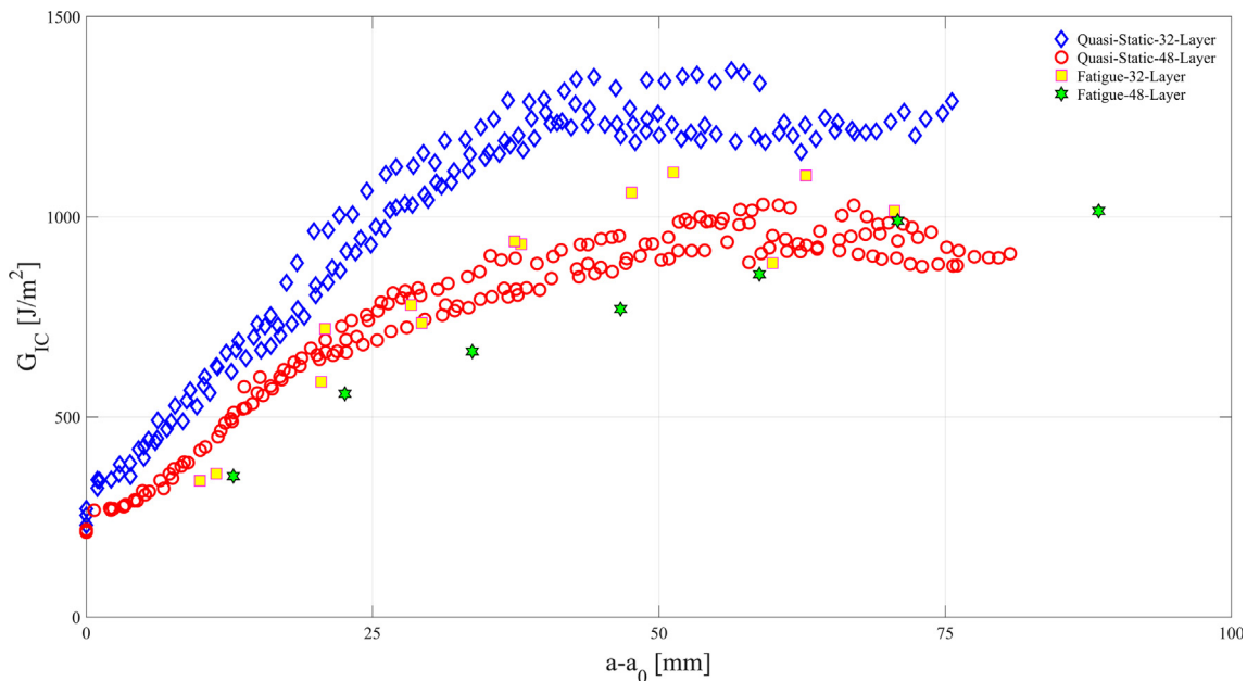
Fig. 7. Quasi-static and fatigue R-curves. (For interpretation of the references to colour in this figure legend, the reader is referred to the web version of this article.)
