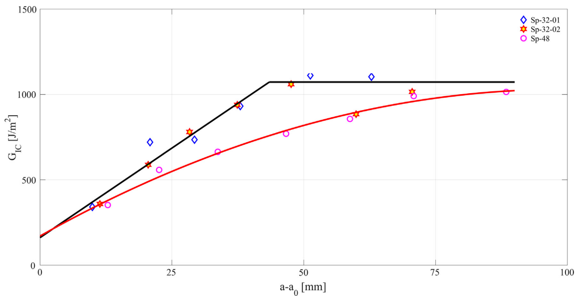
Fig. 5. Fatigue delamination resistance increase. (For interpretation of the references to colour in this figure legend, the reader is referred to the web version of this article.)
