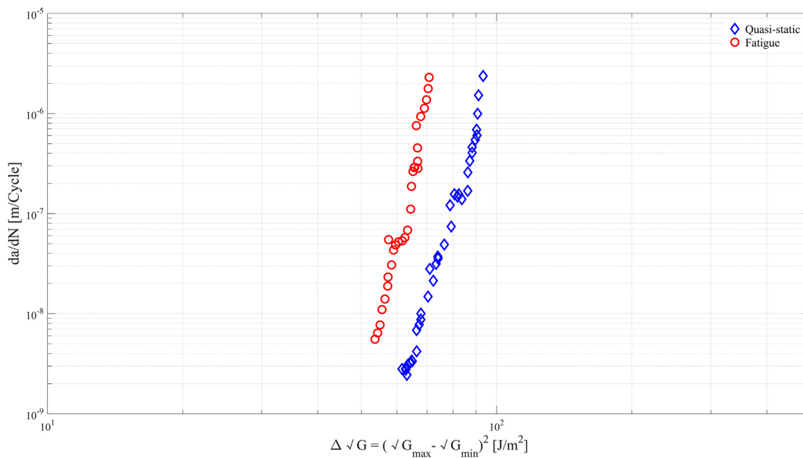
Fig. 10. The difference of fibre bridging in quasi-static and fatigue delamination. (For interpretation of the references to colour in this figure legend, the reader is referred to the web version of this article.)
