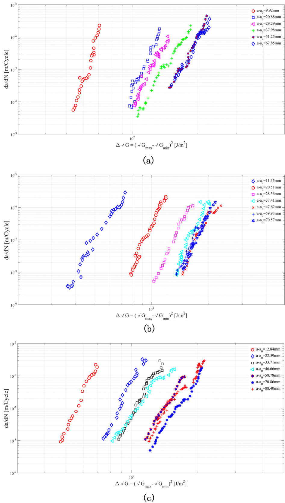
Fig. 8. The Paris representation of fatigue delamination with fibre bridging (a) Sp-32-01; (b) Sp-32-02; (c) Sp-48. (For interpretation of the references to colour in this figure legend, the reader is referred to the web version of this article.)
