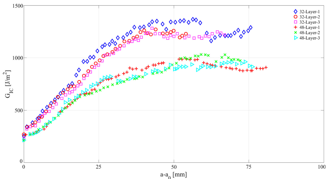
Fig. 2. Quasi-static delamination resistance increase. (For interpretation of the references to colour in this figure legend, the reader is referred to the web version of this article.)
