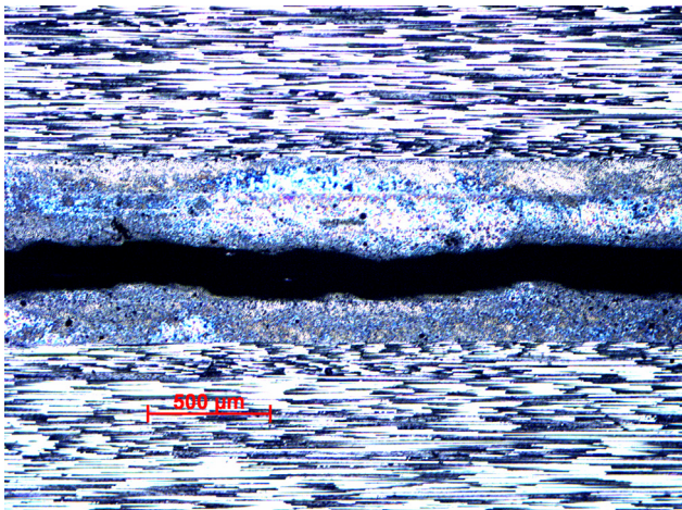
Fig. 6. Fatigue crack profile of multidirectional composite laminates with 32 layers. (For interpretation of the references to colour in this figure legend, the reader is referred to the web version of this article.)
