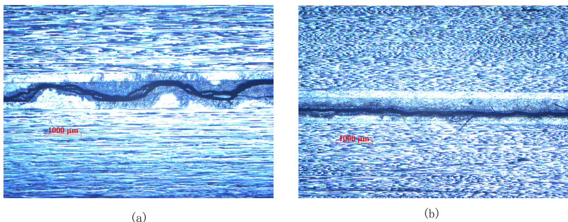
Fig. 3. Quasi-static crack profiles in multidirectional composite laminates (a) 32-Layer; (b) 48-Layer. (For interpretation of the references to colour in this figure legend, the reader is referred to the web version of this article.)
