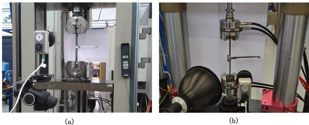
Fig. 1. Quasi-static and fatigue experimental setups (a) Quasi-static experimental setup; (b) Fatigue experimental setup. (For interpretation of the references to colour in this figure legend, the reader is referred to the web version of this article.)
