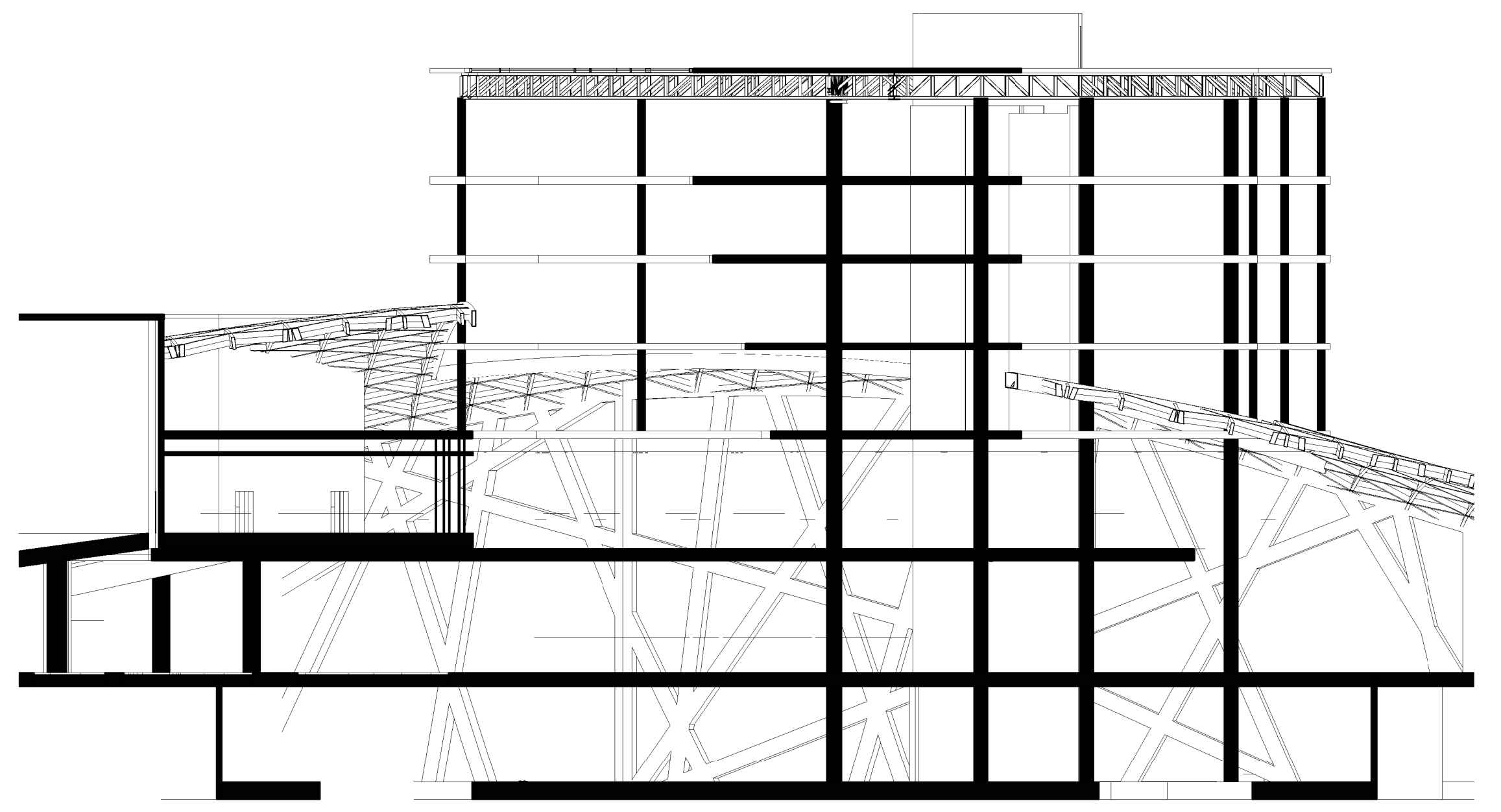
SECTION
