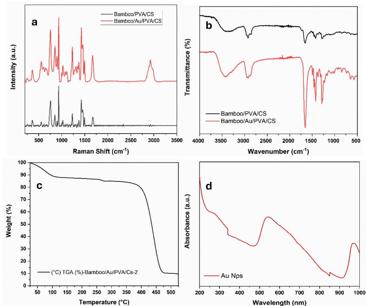
Fig. 2. (a) Raman spectra of Bamboo/PVA/CS and Bamboo/Au/PVA/CS-2 nanofibers. (b) FT-IR spectra of Bamboo/PVA/CS and Bamboo/Au/PVA/CS-2 nanofibers. (c) Thermogravimetric analysis (TGA) curve of Bamboo/Au/PVA/CS-2 nanofibers. (d) UV-Vis absorption spectrum of Au nanoparticles (Au NPs) produced by fs laser ablation.
