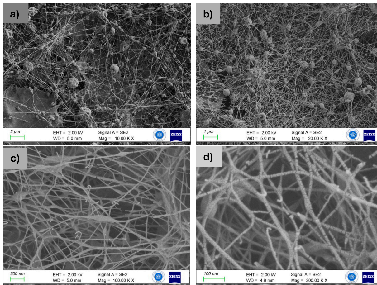
Fig. 3. FE-SEM images of electrospun nanofibers: (a) Bamboo/Au/PVA/CS-1 (10,000 \times ), (b) Bamboo/Au/PVA/CS-2 (20,000 \times ), (c) Bamboo/PVA/CS (100,000 \times ), and (d) PVA/CS (300,000 \times ). Scale bars: (a) 2 \mu m, (b) 1 \mu m, (c) 200 nm, (d) 100 nm.
