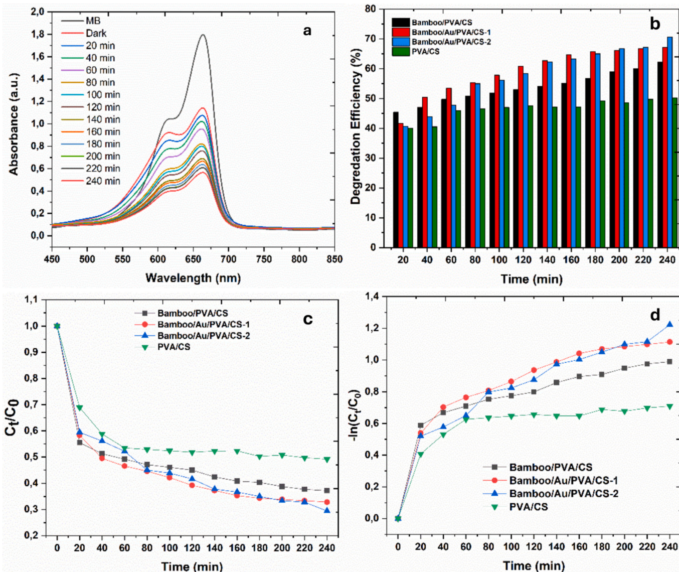
Fig. 4. Photocatalytic degradation of methylene blue (MB) under visible-light irradiation using PVA/CS-based nanofiber photocatalysts. (a) UV-Vis spectra of MB solution at different irradiation times in the presence of Bamboo/Au/PVA/CS-2 nanofibers. (b) Time-dependent photocatalytic degradation efficiency for Bamboo/Au/PVA/CS-1, Bamboo/Au/PVA/CS-2, Bamboo/PVA/CS, and PVA/CS nanofibers. (c) Plots of C_t/C_0 versus irradiation time. (d) Pseudo-first-order kinetic plots, -\ln(C_t/C_0) versus time, were used to determine the apparent rate constants. (For interpretation of the references to colour in this figure legend, the reader is referred to the web version of this article.)
