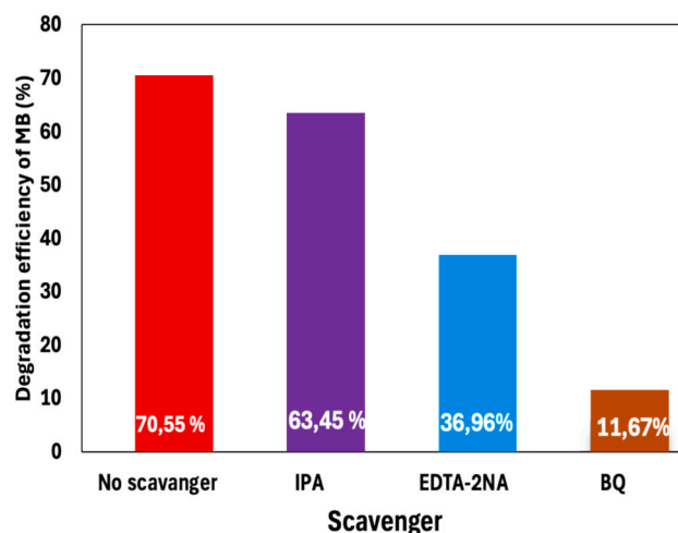
Fig. 5. Effect of different radical scavengers on the photocatalytic degradation of methylene blue (MB) over Bamboo/Au/PVA/CS-2 nanofiber photocatalyst after 240 min of visible-light irradiation: no scavenger, isopropyl alcohol (IPA, \bullet\text{OH} scavenger), ethylenediaminetetraacetic acid disodium salt (EDTA-2Na, \text{h}^+ scavenger), and p-benzoquinone (BQ, \text{O}_2^- scavenger). (For interpretation of the references to colour in this figure legend, the reader is referred to the web version of this article.)
