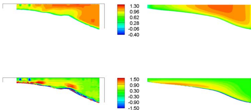
Figure 18. Patterns of the (top) normalized streamwise velocity v_s/U and (bottom) streamwise vorticity \omega_s/(H/U) in the cross-section at 180^\circ in the bend with equilibrium bed. Comparison between (left) measurements and (right) predictions over the fixed prescribed measured equilibrium bathymetry.
