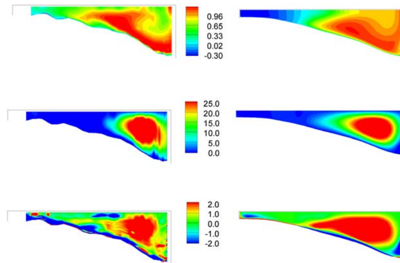
Figure 17. Patterns of the (top) normalized streamwise velocity v_s/U , (middle) normalized cross-stream circulation 100\psi/(UH) , and (bottom) streamwise vorticity \omega_s/(H/U) in the cross-section at 90^\circ in the bend with equilibrium bed. Comparison between (left) measurements and (right) predictions over the fixed prescribed measured equilibrium bathymetry.
