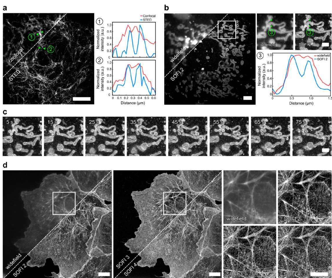
Figure 5. Super-resolution microscopy with HDyes. (a) Live-cell confocal and STED microscopy of COS-7 cells expressing pVimentin N116TAG-BCN labeled with HD653 with intensity line profiles showing the resolution improvement. Scale bar 5 \mu\text{m} . (b) Live-cell widefield (temporal average of series) and second-order SOFI of mitochondria in COS-7 cells transiently expressing TOMM20-mCherry-HaloTag labeled with sb-HD656 via HTL-BCN. Scale bar 5 \mu\text{m} . The close-ups correspond to the ROI indicated in the overview image. The cross-sectional profile of the averaged widefield image and second-order SOFI shows the improved image contrast and resolution. Scale bar 2 \mu\text{m} . (c) Time course of second-order SOFI corresponding to the ROI indicated in (b) showing the movement of mitochondria with a time resolution of 10 s (see Figure S28 for the full sequence). Image acquisition: 500 frames per time point, 20 ms exposure time, 635 nm laser, 140 W/cm 2 . The images are representative of more than five cells from two independent experiments. (d) High-order SOFI imaging of sb-HD656 labeled F-actin in fixed COS-7 cells showing SOFI analysis up to fourth cumulant order. Image acquisition: 20 000 frames, 50 ms exposure time, 635 nm laser, 275 W/cm 2 . The images are representative of six cells from two independent experiments. Scale bars 10 \mu\text{m} .
