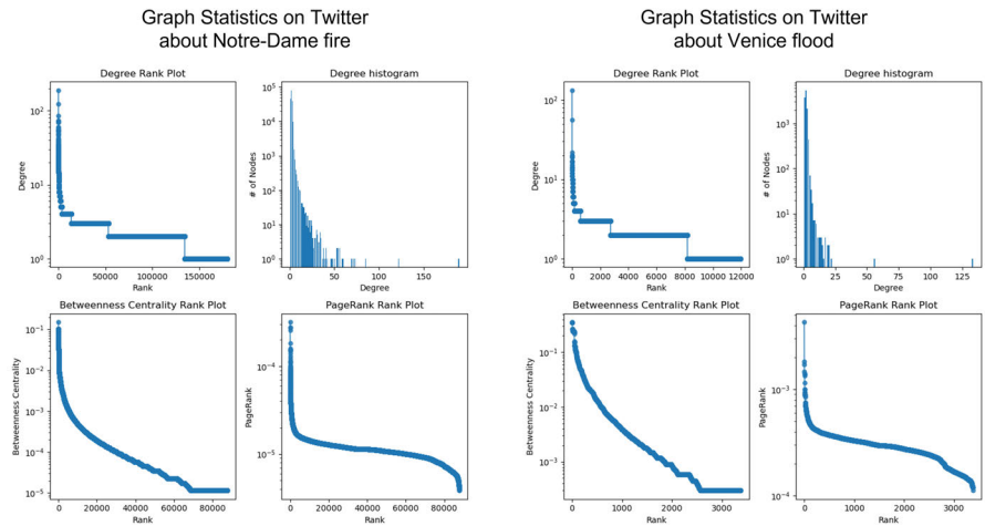
FIG. 6.6 The graph statistics on the conversation graph and/or its largest weakly-connected component in Notre-Dame and Venice, which includes: the log-scale rank-size plot of degree distribution in the entire graph, the log-scale degree histogram, the log-scale rank-size plot of the betweenness centrality on the largest component, and the log-scale rank-size plot of PageRank on the largest component.
