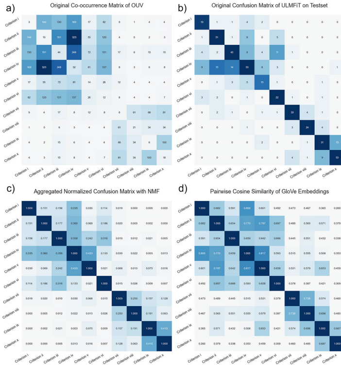
FIG. 3.6 The matrices representing the pairwise similarity and associations between selection criteria. a) the original (unnormalized) co-occurrence matrix A ; b) the original (unnormalized) confusion matrix C^{(4, \text{test})} by m_4 ULMFiT; c) the aggregated normalized confusion matrix constructed from the NMF vector \beta ; d) the semantic similarity matrix H of the pairwise cosine similarity of GloVe embeddings for each criterion.
