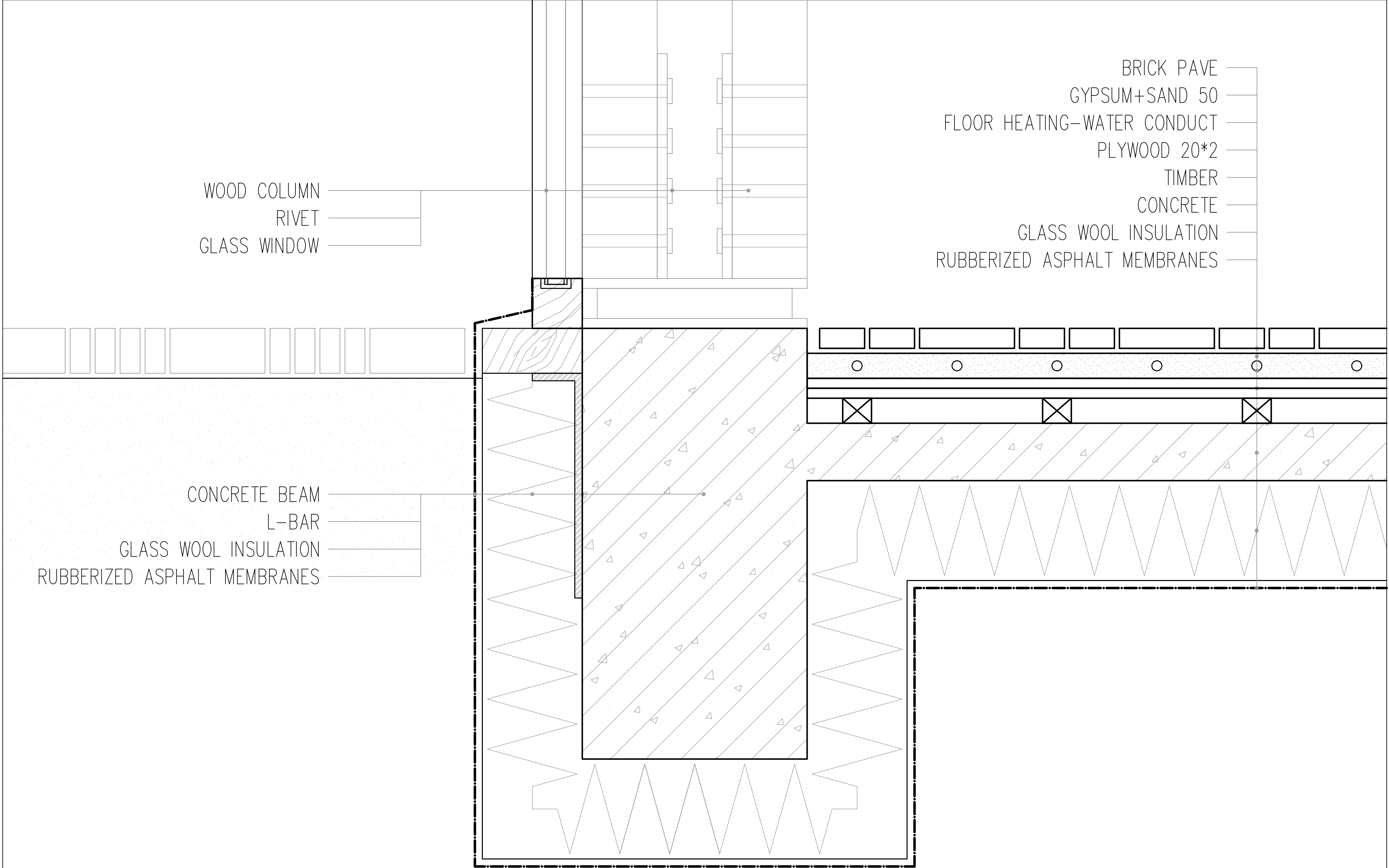
1:5 DETAIL DRAWING-01
