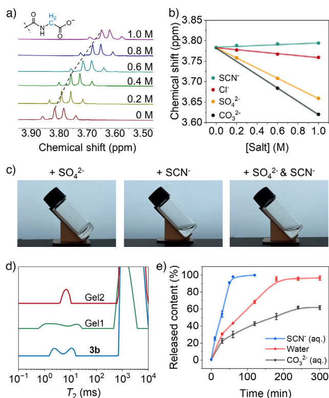
Figure 3. Mechanistic study of the Hofmeister effect-mediated self-assembly of 3b . a) 1 H NMR spectra of glycine methylene in 3b at different [\text{CO}_3^{2-}] , pD = 8.0. b) 1 H NMR chemical shifts of the glycine methylene in 3b against the concentration of different anions. c) Photographs showing the hydrogelation behavior of 3b in the presence of \text{SO}_4^{2-} , \text{SCN}^- , and \text{SO}_4^{2-} + \text{SCN}^- , respectively. (d) Low-field 1 H NMR spectra of gelator 3b , Gel1, and Gel2. e) Disintegration of Gel2 triggered by diffusion of \text{CO}_3^{2-} and the addition of \text{SCN}^- for controlled release of model drug bromocresol purple (2.0 mM), error bars represent SD from three independent experiments. Samples: [ 3b ] = 15 mM in (a) and b) and 60 mM in (c)–(e); unless stated otherwise, [salt] = 1.0 M.
