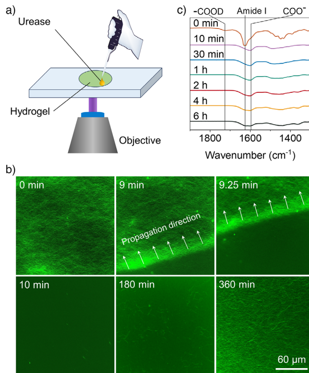
Figure 5. Mechanic insight into the dynamic gel-sol-gel transition process. a) Experimental setup for the in situ confocal microscopy observations. b) Confocal images showing the dynamic evolution process of the hydrogel networks. c) Time-dependent FTIR spectra probing the dynamic evolution of molecular structures and intermolecular interactions of gelator 3 . Samples: initial pH 5.0, [3a] = 60 mM, [urea] = 1.0 M, [urease] = 0.16 \text{mg mL}^{-1} .
