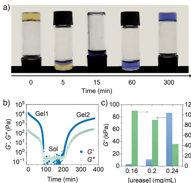
Figure 4. Hofmeister effect-mediated dynamic gel-sol-gel transition. a) Time-dependent gel-sol-gel transition process triggered by urease with 50 \mu\text{M} bromocresol purple as a pH indicator. b) Time-sweep rheological test showing the dynamic gel-sol-gel transition process. c) Stiffness of Gel2 and transition time at different [urease]. Samples: initial pH 5.0, [3a] = 60 mM, [urea] = 1.0 M, [urease] = 0.16 \text{mg mL}^{-1} .
