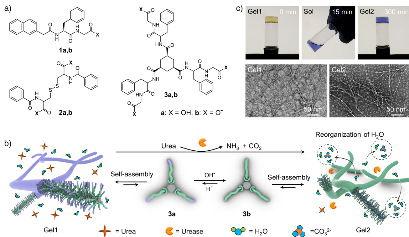
Figure 1. Hofmeister effect-mediated dynamic supramolecular hydrogelation. a) Chemical structures of gelators 1 , 2 , and 3 . b) Illustration of the self-assembly of gelator 3 into Gel1 through protonation, and the transition process from Gel1 to sol, and eventually to Gel2 relying on the enzymatic production of basic NH 3 and kosmotropic ions, NH 4 + and CO 3 2- . c) Typical sample showing the dynamic gel-sol-gel transition process and the TEM images of Gel1 and Gel2 of gelator 3 . Sample in (c): initial pH 5.0, [3a] = 60 mM, [urea] = 1.0 M, [urease] = 0.16 mg mL -1 , and [bromocresol purple] = 50 μM (pH indicator).
