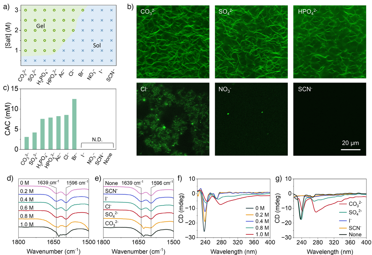
Figure 2. Self-assembly of gelator 3b driven by kosmotropic anions. a) Hydrogelation diagram in the presence of different anions. b) Confocal microscopy images showing the self-assembled structures of gelator 3b , [ 3b ] = 30 mM. c) CAC of 3b in the presence of different anions, N.D. means not detected. FTIR spectra of gelator 3b in the presence of d) varying [ \text{CO}_3^{2-} ] and e) different anions. CD spectra of gelator 3b in the presence of f) varying [ \text{CO}_3^{2-} ] and g) different anions, [ 3b ] = 5 mM. Unless stated otherwise, [salt] = 1.0 M and [ 3b ] = 60 mM at pH 8.0.
