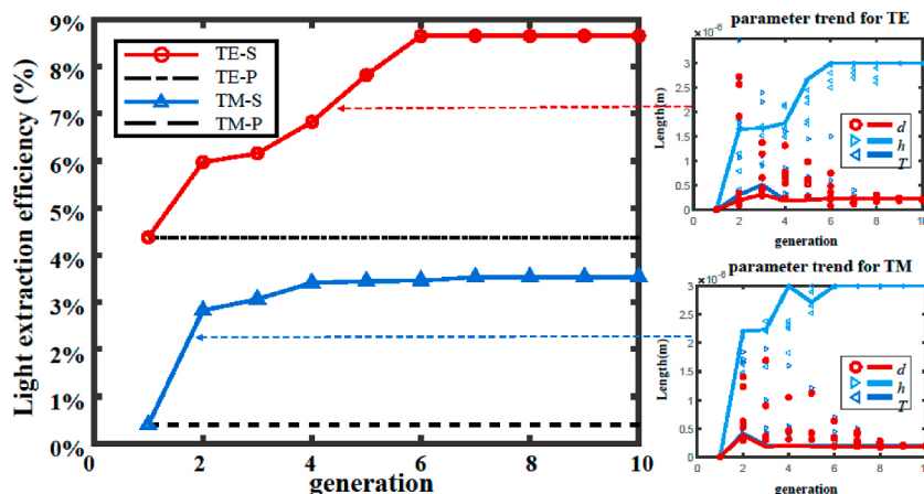
Fig. 3. Optimization process of the surface microstructure based on parabola cone array to improve light exaction and adjustment process of the structure parameter value with generation, TE/TM-S: optimized surface structure for TE/TM-polarized emission, TE/TM-P: planar structure for TE/TM-polarized emission.
