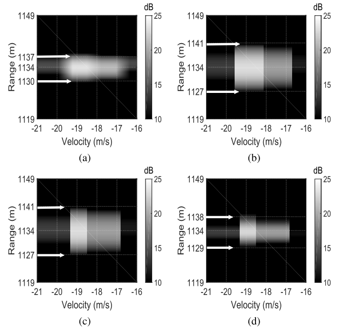
Fig. 11. Range-Velocity results maps for the automobile in the experiment described in Section. V-C. (a) As seen in the 40 MHz channel. (b) As seen in the 20 MHz channel. (c) Processing with manually discarding every other sweep of the 20 MHz channel. (d) Processing the 20 MHz waveform with a concatenation factor d = 2 , the automobile's resolution closely match that of the 40 MHz waveform, in range, velocity and SNR.
