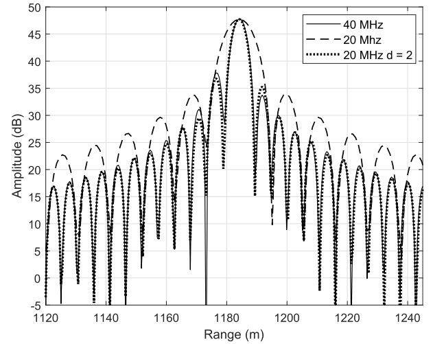
Fig. 10. Zero-Doppler cut zoom-in on the Chimney shown in Fig. 8 (a) and (b). The proposed processing of the 20 MHz channel - with a concatenation factor d = 2 - closely matches that of the 40 MHz channel. The sub-chimneys are resolvable, as can be seen in the disbalanced shape of the sinc-function.
