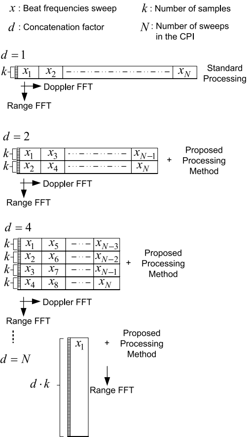
Fig. 3. Reconfigurable range-Doppler processing permutations of fast-time slow-time received sweeps. The total CPI processing gain is maintained. Depending on the number of sweeps concatenated, there is a tradeoff between range resolution and the maximum unambiguous Doppler velocity interval. Note that when d = N , only a range profile is provided because the matrix is then one dimensional.
