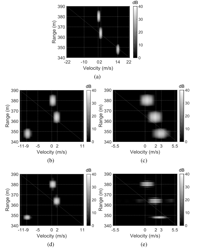
Fig. 7. Simulation Results for the scenario setup using the parameters in Table II and illustrated in Fig. 6. (a) Standard processing, PRF = 1 \text{ kHz} . (b) Dropped sweeps to create PRF = 500 \text{ Hz} . (c) Dropped sweeps to create PRF = 250 \text{ Hz} . (d) Proposed processing with d = 2 . (e) Proposed processing with d = 4 .
