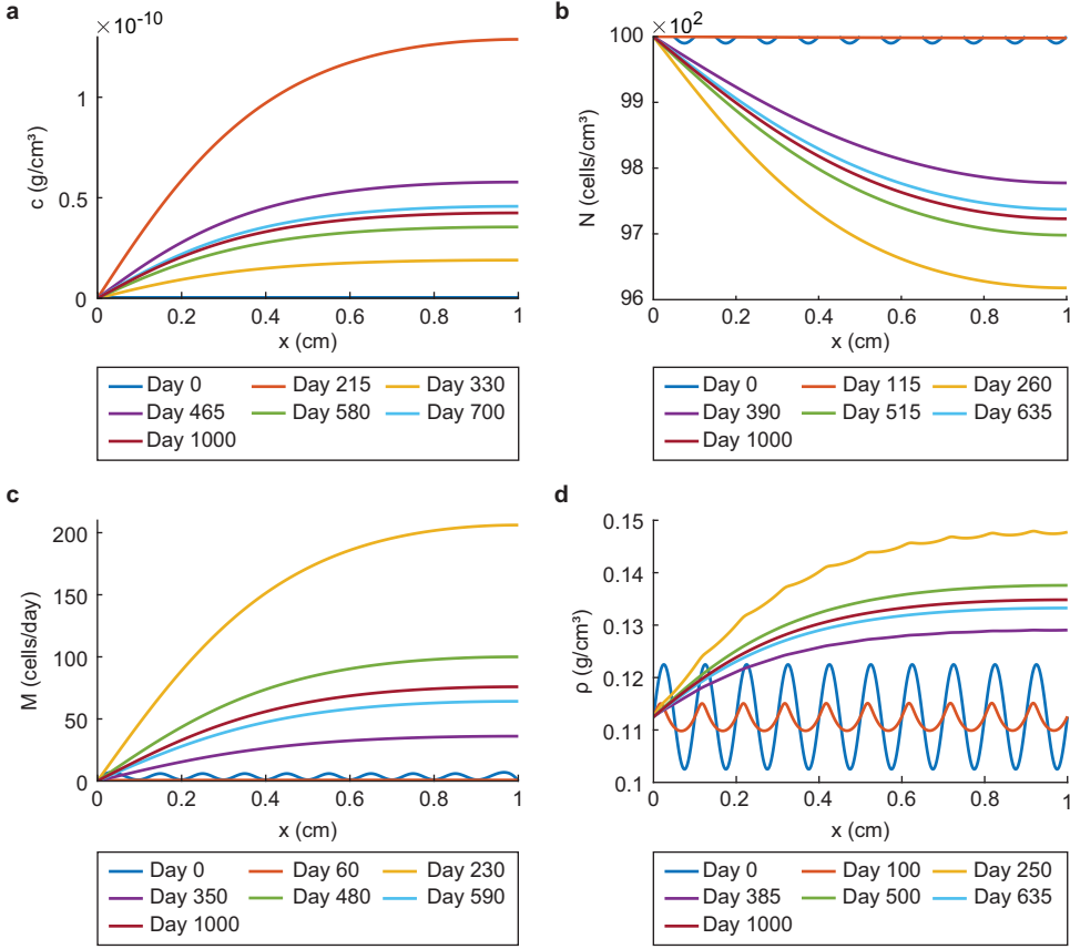
Figure 3.5: Evolution of the perturbed chemical densities for \delta_c = 3 \times 10^{-4} \text{ cm}^6/(\text{cells g day}) and \mu = 100 \text{ (N day)/cm}^2 and k = 10 . The plots show the signaling molecules (a), the fibroblasts (b), the myofibroblasts (c), and collagen (d).
