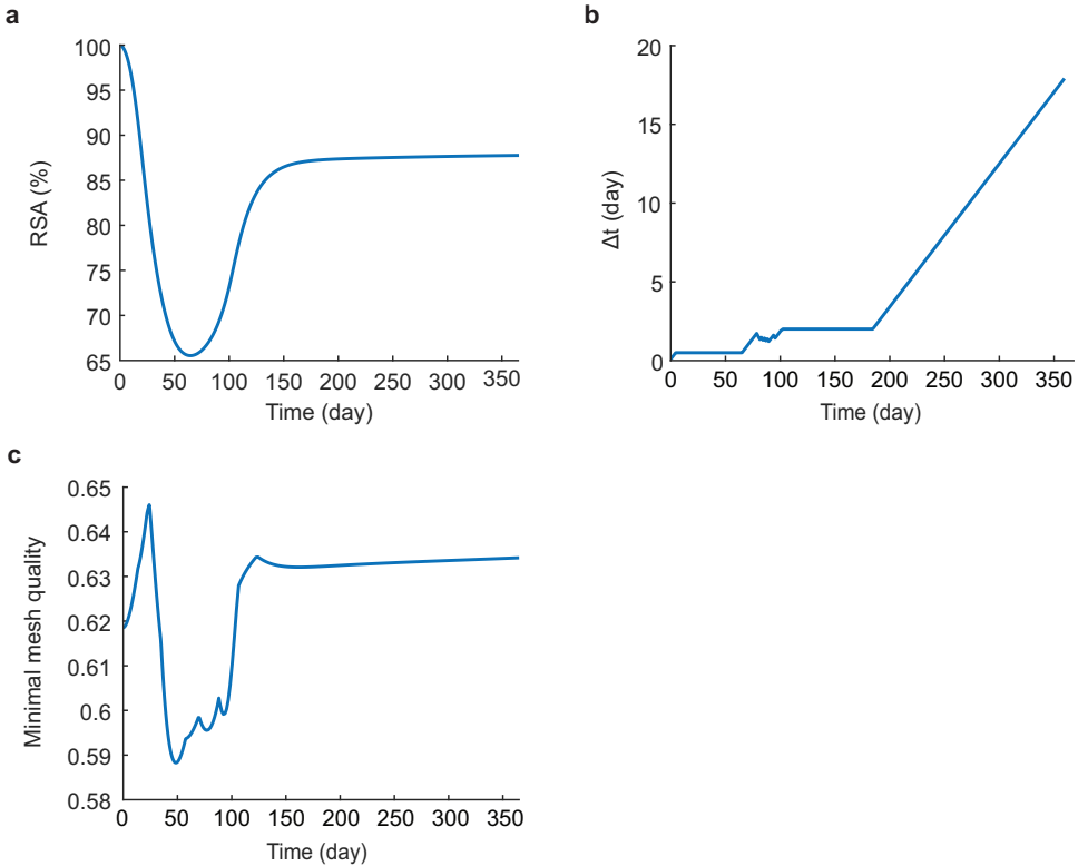
Figure 6.2: Examples of the evolution of the RSA (a), the variable timestep (b), and the mesh quality (c) during a simulation.
