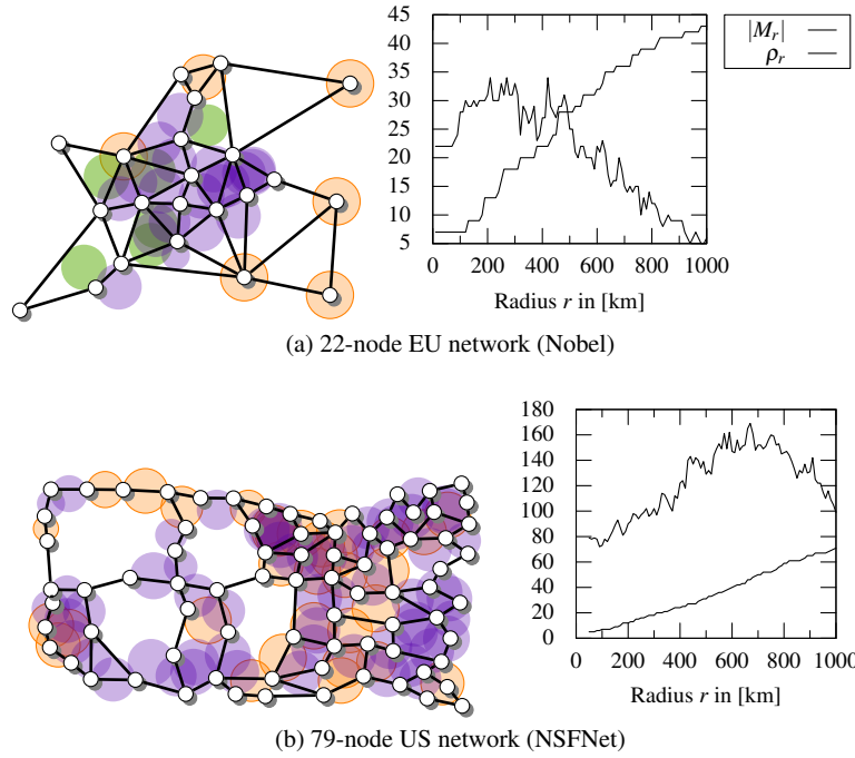
Fig. 7: Simulation results for determining list M_r of maximal SRLGs of disasters being circular disks with radius r .
