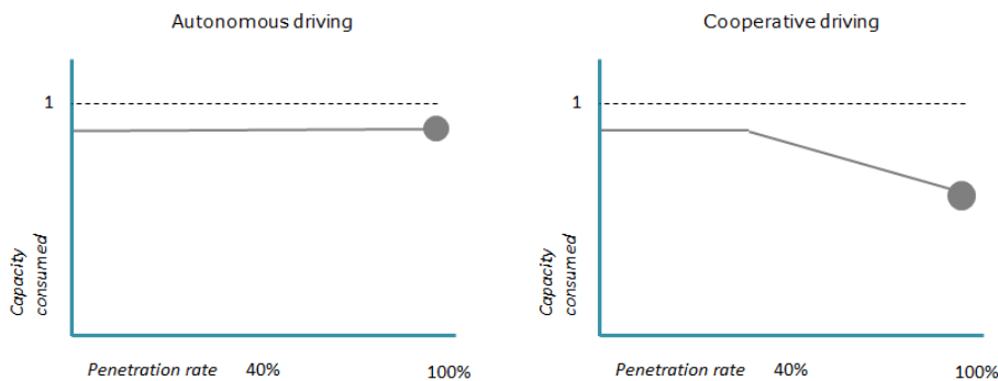
FIGURE 2 PCUA value for different penetration rate for autonomous and cooperative driving (van Arem et al., 2006; Arnaout and Bowling, 2011; Ngoduy et al., 2009; Wilmink et al., 2014).
