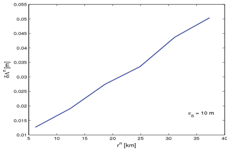
Figure 4-9 | Worst-case error in phase synchronization as a function of the lateral separation for an error of 10 m in the estimated position of the satellite .
