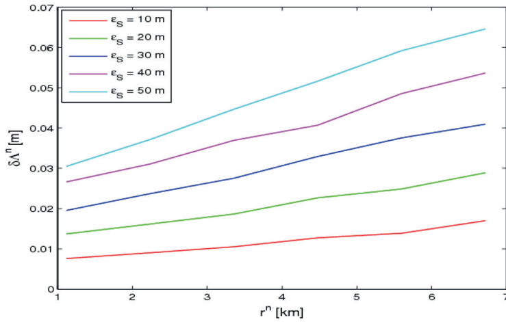
Figure 4-12 | Worst-case error in phase synchronization \delta A^n as a function of the lateral separation r^n for different error levels in the estimated position of the satellite S^n
