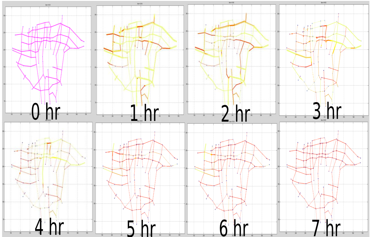
Figure 3 Evolution of gridlocks over time and space for 2 hours loading duration (red color represents zero velocity).
