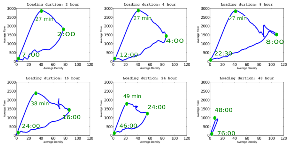
Figure 4 Network Fundamental Diagram for different loading durations
