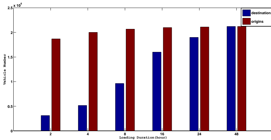
Figure 2 Number of vehicles at origins and destinations for different evacuation cases
