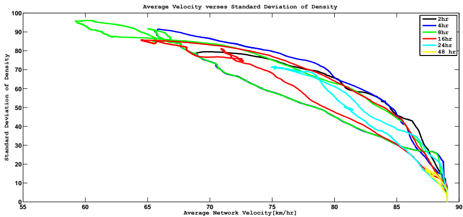
Figure 6 Standard deviation of densities versus average network velocity for all loading cases.
