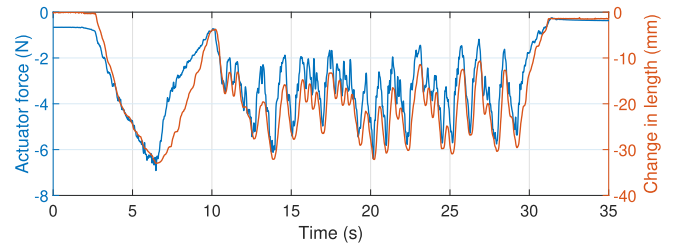
Fig. 5. Actuator force and length variation.
