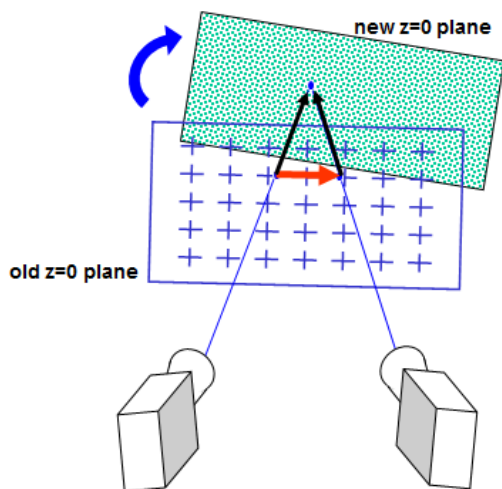
Figure 3.3. Stereo-PIV self-calibration procedure correcting misalignment of laser sheet.
