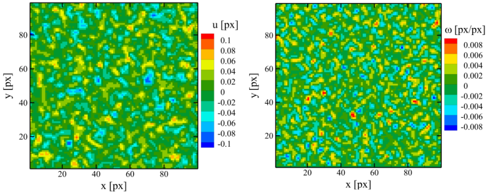
Figure 4.4. Instantaneous horizontal velocity (left) and vorticity fields (right) for the case U = 0.1 px and \rho = 0.45 .
