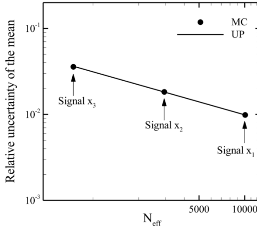
Figure 4.7. Uncertainty of the mean value (relative to the standard deviation) as a function of the effective number of samples N_{eff} . Comparison between Monte Carlo simulation results (MC) and theoretical uncertainty propagation (UP).
