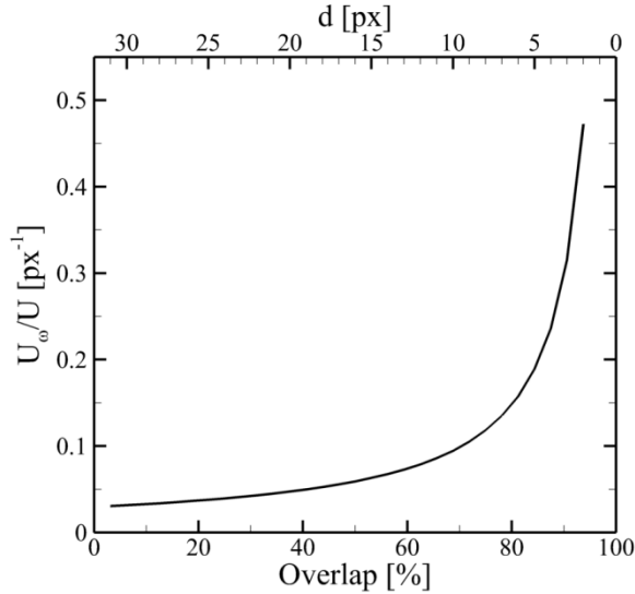
Figure 4.1. Uncertainty of the vorticity as a function of the interrogation window overlap. Results for interrogation window of size 32 \times 32 px 2 .
