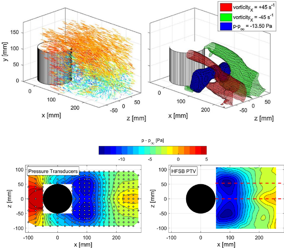
Figure 8.2. Pressure computation from Tomographic PTV data using HSFB. Particle tracks, vorticity and pressure (top) and comparison of surface pressure to pressure transducer values (bottom). From Schneiders et al. (2016c).
