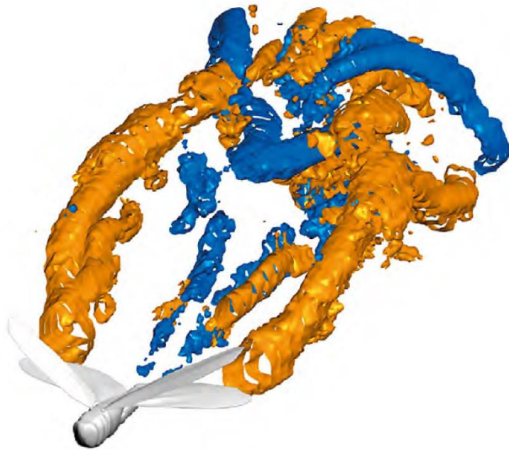
Figure 1.3. Instantaneous vortex pattern using time-resolved tomographic PIV behind a locust (from Bompfrey et al. 2012).
