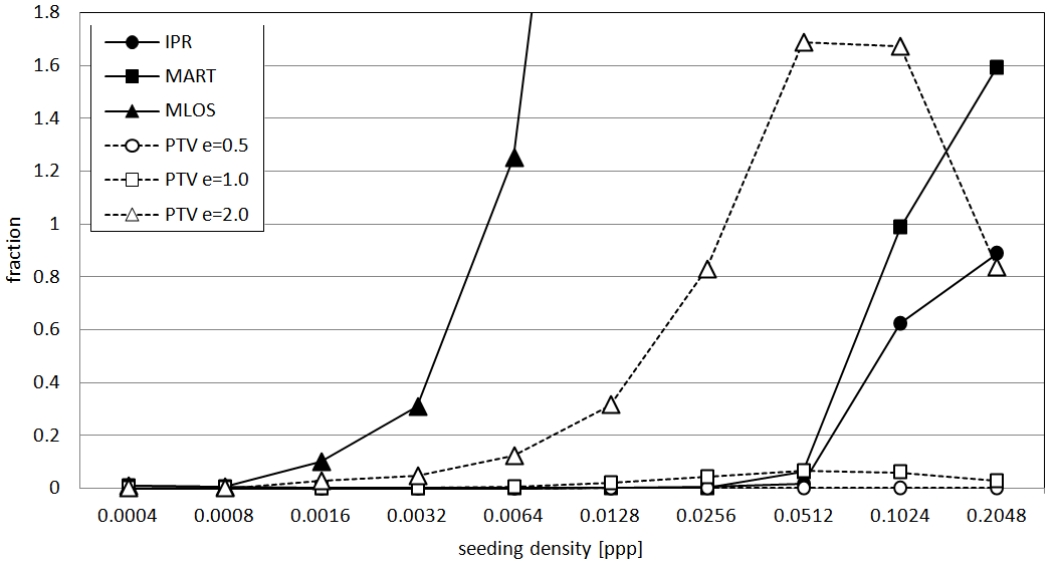
Figure 7.6. Fraction of ghost particles.
