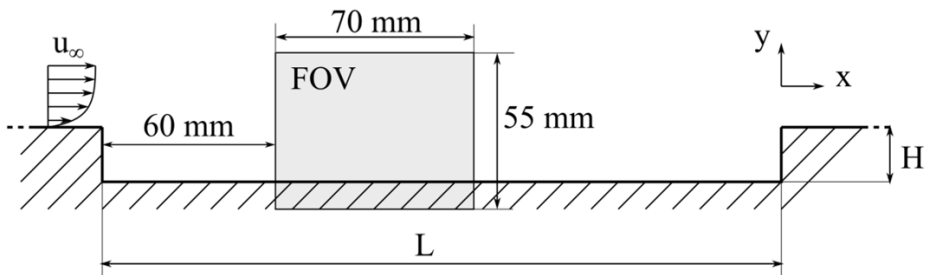
Figure 4.11. Sketch of the cavity flow experiment.
