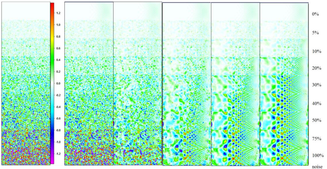
Figure 5.6. Original noise and after denoising (equal to Figure 5.5 minus Figure 5.4 middle) with strength S = 1, 2, 2.5, 3 , and 4 from left to right. Noise level 0-100\% from top to bottom. Color = u -component of noise.
