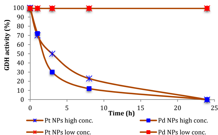
Figure 1. GDH activity over time in the presence of Pt and Pd NPs, at different NPs concentrations. (NPs low conc.: 10 \mu L of 5.64 \times 10^{-3} M Pd NPs or 5 \mu L of 9.66 \times 10^{-3} M Pt NPs, with 4 mg of GDH similar to the same ratio used in the reaction carried out in autoclave; NPs high conc.: 100 \mu L of 5.64 \times 10^{-3} M Pd NPs or 50 \mu L of 9.66 \times 10^{-3} M Pt NPs, with 4 mg of GDH) (see experimental).
