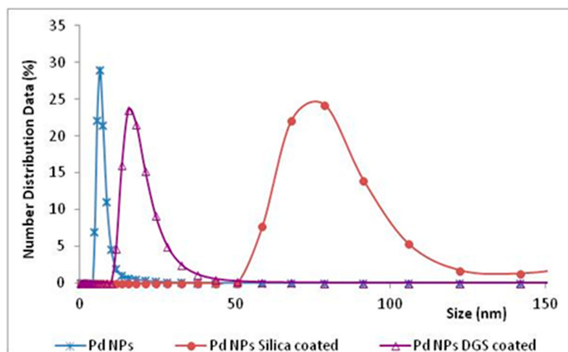
Figure 9. DLS spectra of Pd NPs solution (8 nm); DGS-coated Pd NPs (16 nm); silica-coated Pd NPs (80 nm).
