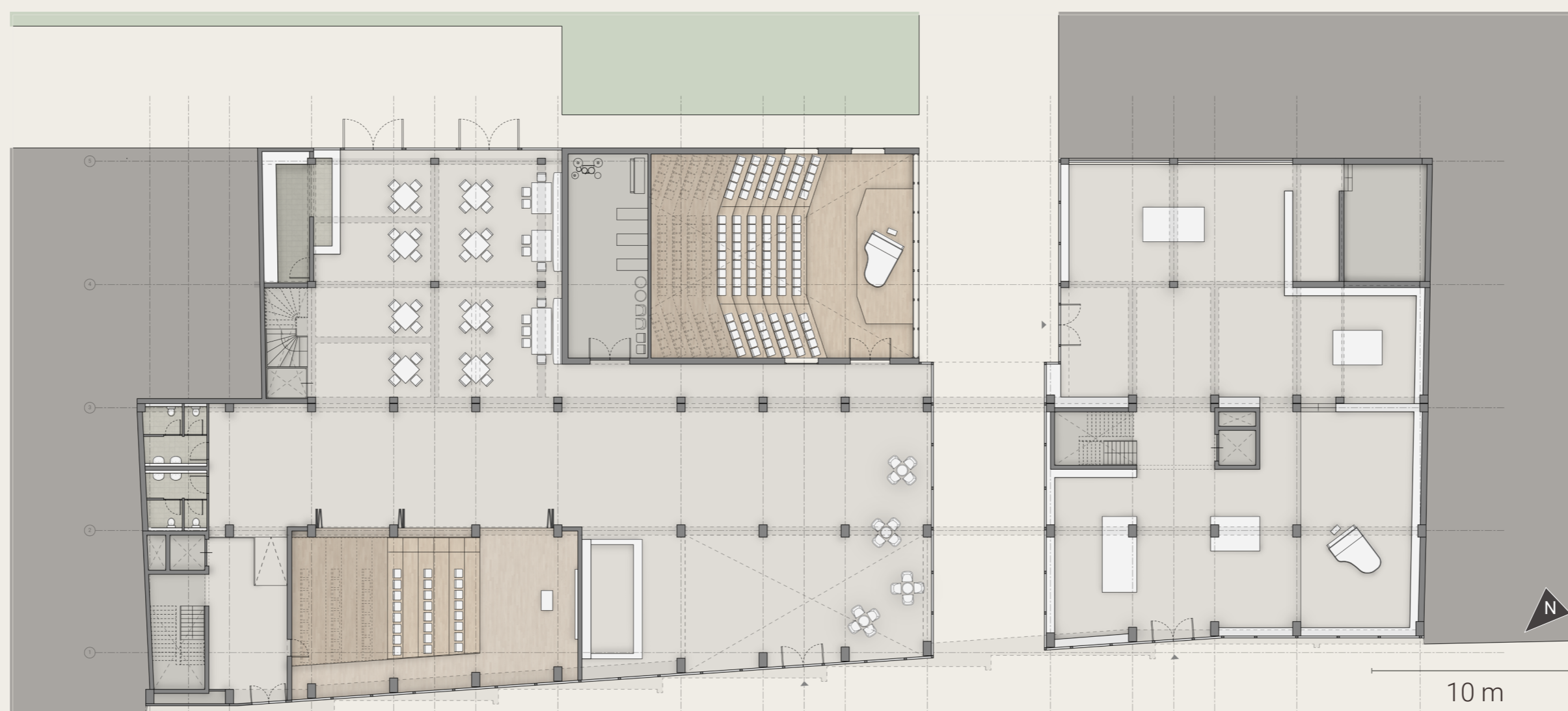
GROUND FLOOR
