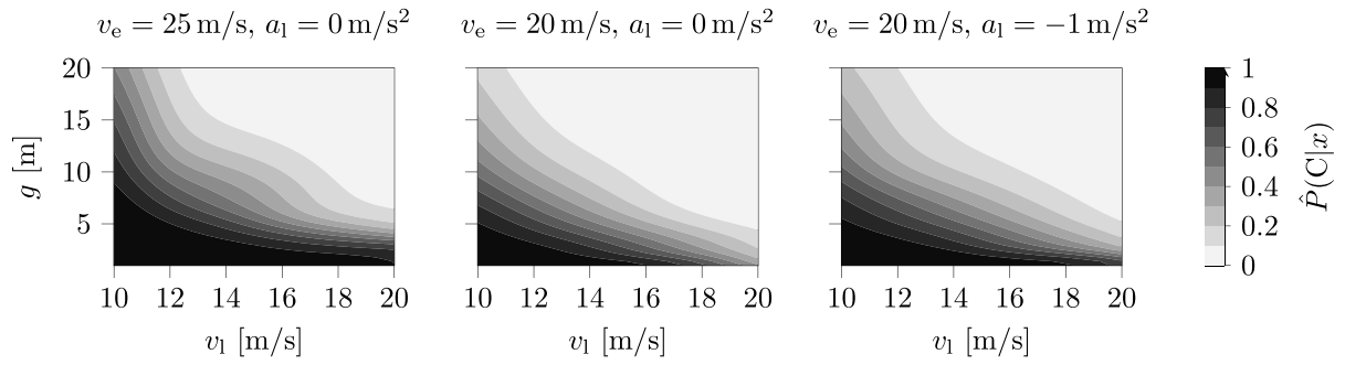
Fig. 4. Heat maps of the SSM described in Section 4.2 as a function of the speed of the leading vehicle ( v_l ) and the gap between the ego vehicle and the leading vehicle ( g ). For each heat map, the other two input parameters are fixed at v_e = 25 m/s (left) or v_e = 20 m/s (center and right) and a_l = 0 m/s 2 (left and center) or a_l = -1 m/s 2 (right). The estimated crash probability ranges from 0 (white) to 1 (black).
