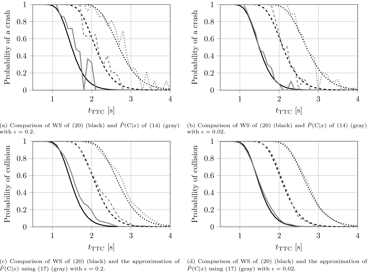
Fig. 2. Comparison of WS of (20) (black lines) and \hat{P}(C|x) of (14) (a,b) or the approximation of \hat{P}(C|x) using (17) (c,d) (gray lines) for a speed difference of \Delta v = 10 m/s (solid lines), \Delta v = 20 m/s (dashed lines), and \Delta v = 30 m/s (dotted lines). Here, \hat{P}(C|x) is based on the same underlying assumptions as WS, see Section 4.1.1. The influence of the parameter \epsilon , which determines the number of simulations to estimate P(C|x) , is illustrated by using different values.
