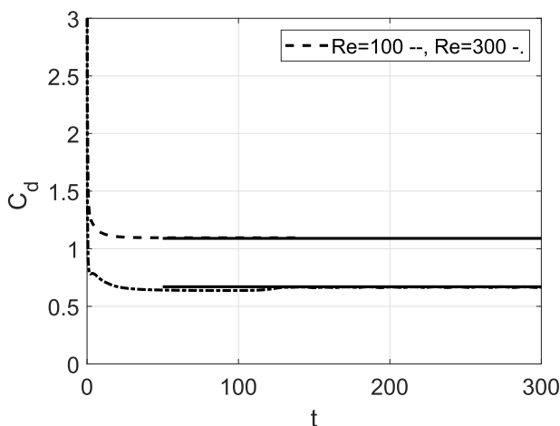
FIG. 22. Comparison of C_d as a function of time for Re = 100 and Re = 300 with the literature result [the final literature value of C_d = 1.09 for Re = 100 and C_d = 0.67 (averaged value) for Re = 300 ].
