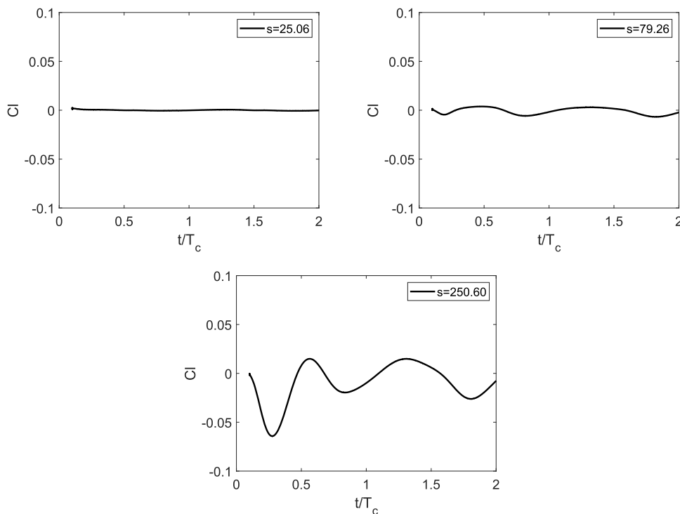
FIG. 18. Numerical results for the dimensionless lift force of the swimmer as a function of dimensionless time for three values of s .
