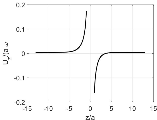
FIG. 5. Instantaneous velocity in the axial direction along the symmetry axis of the swimmer between the points (x/a = 0, y/a = 0, z/a = -15) and (x/a = 0, y/a = 0, z/a = 15) for the left panel of Fig. 4.
