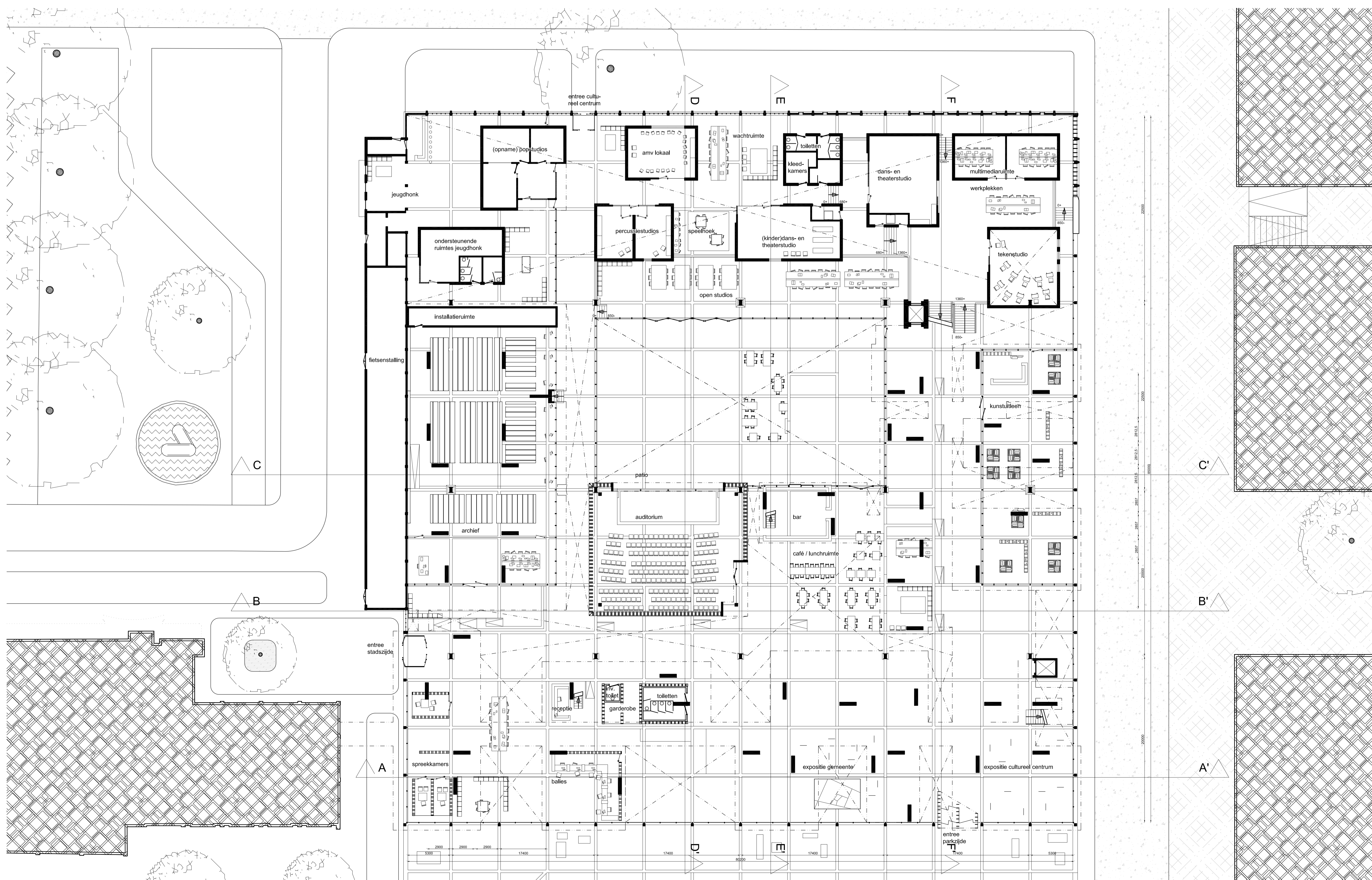
Begane Grond - 1:200
