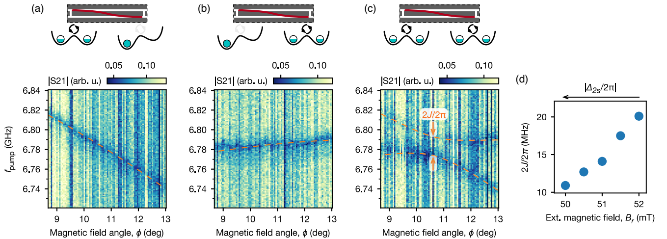
FIG. 3. Spin-spin coupling via virtual photons. (a,b) Dependence of the independently interacting spin transition frequencies as a function of the external magnetic field angle \phi at B_r = 52 mT. See Appendix C for the reconstruction procedure responsible for the vertical stripes. (c) When both spins interact simultaneously with the resonator, an avoided crossing is observed. The spin states hybridize with a splitting 2J/2\pi = 19.0 MHz, larger than any of the transition widths 2\Gamma_s/2\pi \leq (13.2 \pm 4.2) MHz. A dark state is observed along the upper branch, an effect caused by the symmetry of the coherently hybridized spin states. (d) Plot showing how the exchange interaction is reduced when the spin-photon detuning is increased.
