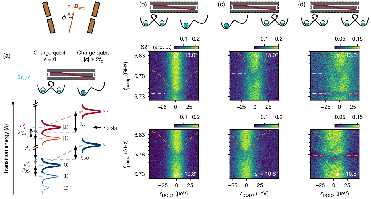
FIG. 8. Dispersive regime transitions, and spin-spin interaction versus DQD detuning. (a) Schematic representation of the transition energy shifts in the dispersive regime. See Appendix D for details. (b,c) Measurement of spin transitions for DQD1 (b) and DQD2 (c) as a function of the charge detuning \epsilon with dispersive readout, with 2t_c/h \approx 8.7 GHz and B_r = 52 mT. A pump tone is sent down the gate lines to excite the spins, resulting in a signal dip when the pump and spin frequencies match. Here, (f_{probe}^1, f_{probe}^2, f_{probe}^{12}) \approx (6.9038, 6.9061, 6.8981) GHz for \phi = 10.8^\circ . The spin transition frequency at \epsilon = 0 \mu\text{eV} is marked with a white dashed line for comparison between plots. (d) When the spins are simultaneously interacting with the resonator, the spin states hybridize depending on their energy difference. In the nonresonant case, \phi = 13.0^\circ , their energies are minimally perturbed, as can be seen by the model lines and the white guides. In the resonant case, \phi = 10.8^\circ , the two spins hybridize due to the exchange interaction 2J/2\pi = 20.2 MHz mediated by virtual resonator photons. The upper state is hardly visible because its symmetry makes it dark to the resonator probe, which is expected for a coherent spin-spin interaction.
