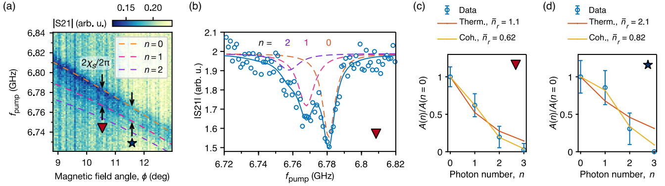
FIG. 4. Photon-number-resolved spin dispersive shift. (a) Spin transition frequency of DQD1 showing an extra dip below the main transition for larger probe power. The dip matches well the prediction from the Hamiltonian model (dashed lines) for |\downarrow, n\rangle \leftrightarrow |\uparrow, n\rangle transitions, with the first two transitions visible in this plot. (b) Line cut of the data in panel (a) for \phi = 10.55^\circ , and fit to four Lorentzian dips (first three shown with dashed lines). A dispersive shift 2\chi_s/2\pi = -13.1 \pm 2.2 MHz is extracted. (c) Relative area of the dips for \phi = 10.55^\circ , and comparison with thermal [ P_{\text{thermal}}(n) = \bar{n}_r^n / (\bar{n}_r + 1)^{n+1} ] and coherent [ P_{\text{coherent}}(n) = e^{-\bar{n}_r} \bar{n}_r^n / n! ] photon-number distributions. The error bar represents the 95% confidence interval. (d) Relative area for \phi = 11.6^\circ . At this angle, the resonator has a smaller \kappa'_r , resulting in a larger steady-state photon number. The coherent-state distribution has better agreement.
