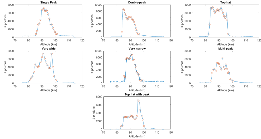
Figure 6. Distribution of the sodium concentration regarding altitude [3]. The blue curve represents the actual data, the orange dots the points used in our simulations. These profiles have approximately the same probability of occurrence.
