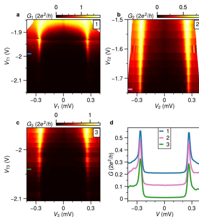
Figure 2. Hard superconducting gap at zero magnetic field. (a–c) Tunneling conductance G_i as a function of individual tunnel gate V_{Ti} and the corresponding applied bias voltage V_i ( i \in \{1, 2, 3\} ). With a substantial change of the out-of-gap state conductance, no discrete subgap states are observed within the gap, indicating clean tunnel junctions. Probe numbers are labeled in the top-right corner. (d) Exemplary line traces indicate the presence of two sharp coherence peaks and a hard induced superconducting gap (the lines are laterally offset by 0.1 G_0 for clarity). The measured lock-in signals are higher than the noise floor due to the additional parasitic capacitance in the circuit, and a detailed comparison with the numerical derivative of the DC current is made in Figure S1. V_{GG} is at -2.6 \text{ V} .
