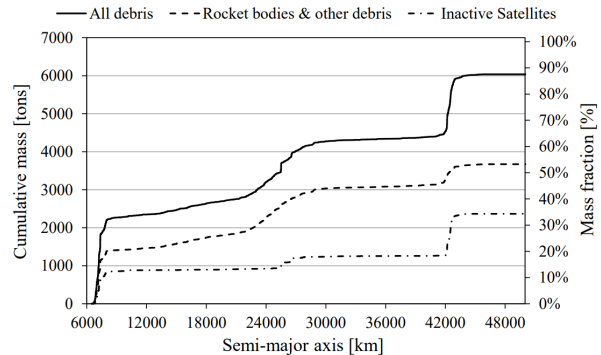
Figure 3. Cumulative mass distribution of the space debris dataset mapped onto debris semi-major axis.
