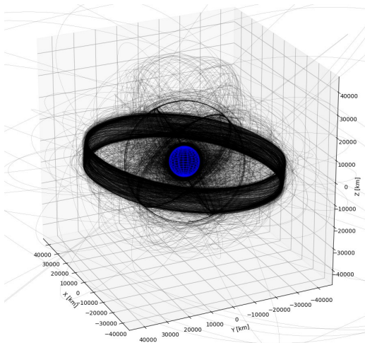
Figure 2. Visualization of debris orbits for all actively tracked space debris objects.
