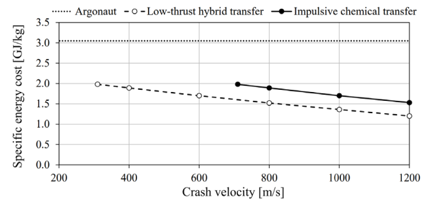
Figure 14. Specific energy cost as function of assumed debris crash velocity onto the Lunar surface.
