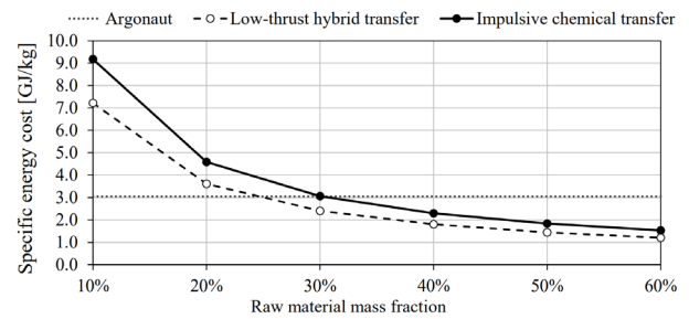
Figure 13. Specific energy cost as function of assumed raw material mass fraction.
