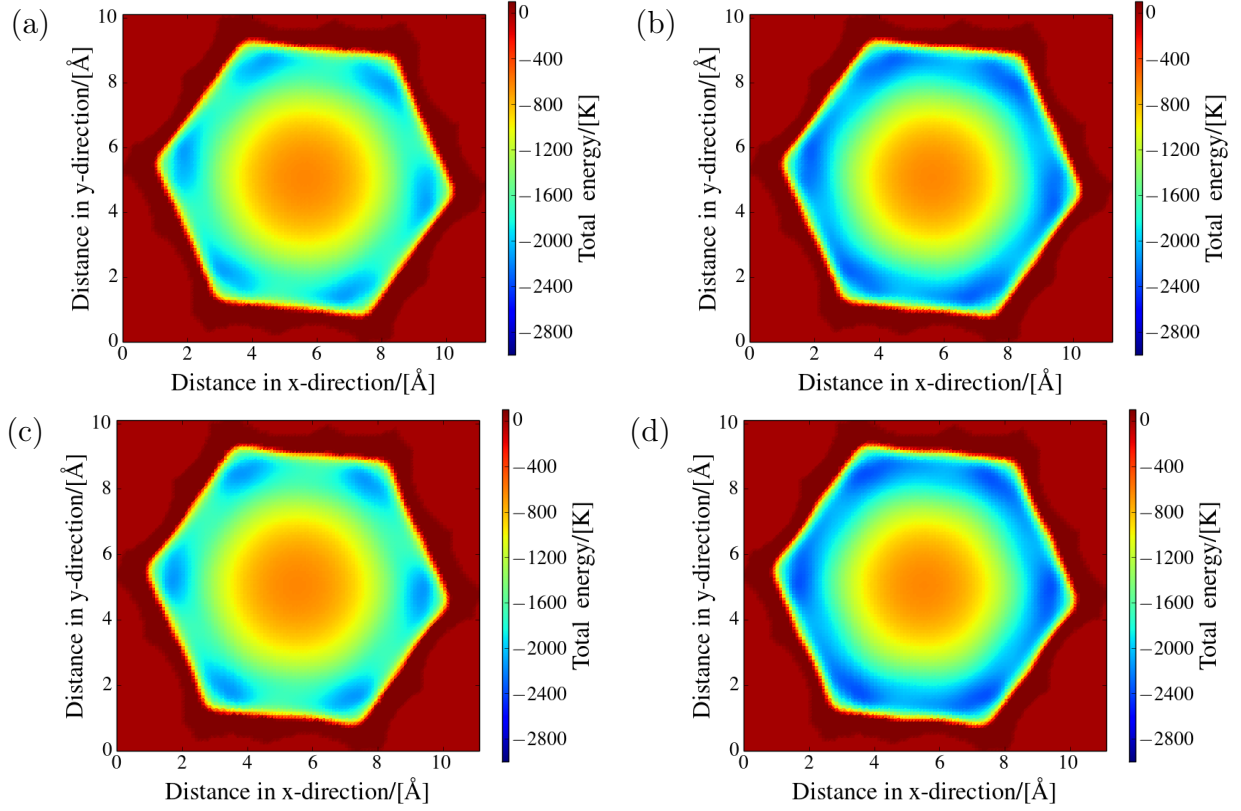
Figure 18: Comparison between the total energies for ethylene in Co-MOF-74 on a grid (left) without and (right) with explicit consideration of polarization energy. Energies calculated with (a) and (b) DFT charges and (c) and (d) charges calculated with the QEq method for the plane of maximum energy. Grid points for which the total energy (in units of k_B ) is larger than 100 K are represented in dark red.
