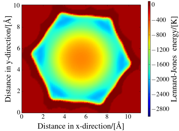
Figure 15: Lennard-Jones energies evaluated on a grid with 0.1 Å spacing on the maximum energy plane in z-direction for ethylene in Co-MOF-74. Grid points for which the total energy (in units of k_B ) is larger than 100 K are represented in dark red.
