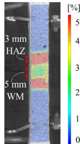
Fig. 13. Measuring range of virtual extensometers in DIC.
