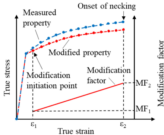
a) Schematic diagram of the linear stress modification factor.
