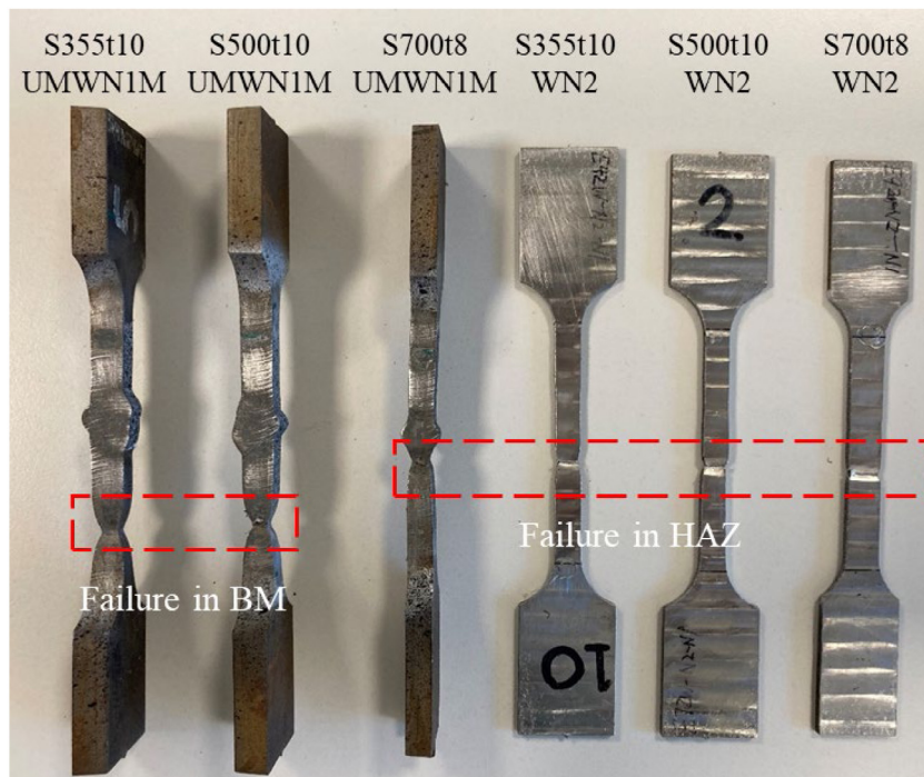
Fig. 16. Failure of milled and unmilled welded coupon specimens.
