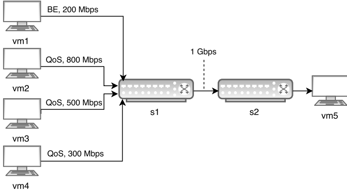
Fig. 4. Topology for the aggregation and prioritization test
