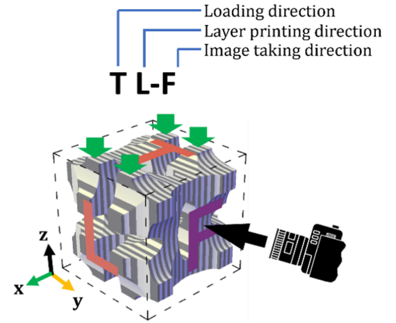
Fig. 6. An example of the notation rule for the tested specimens; it shows this specimen is uniaxial loaded from the top (T) with layers printed from left (L) and pictures taken from front (F); note that the shell was always printed from bottom up, namely the “L” direction was on the printer build plate herein.
