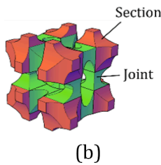
Fig. 2. Schematics of a) creating the 3D auxetic structure, b) definition of the “section” (red regions) and “joint” (green regions). (For interpretation of the references to colour in this figure legend, the reader is referred to the web version of this article.)
