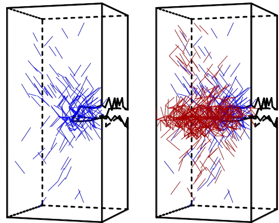
Fig. 13. Simulated crack patterns before peak load (blue elements) and after peak load (red elements). Figures on the left show cracks at maximum load, while on the right they show cracks at failure. (For interpretation of the references to color in this figure legend, the reader is referred to the web version of this article.)
