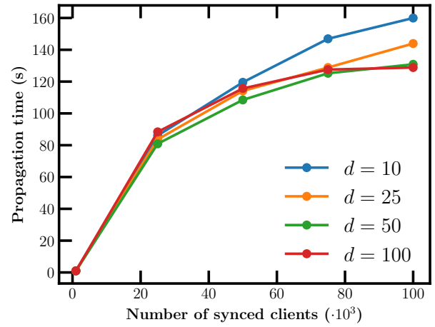
Fig. 3: Revocation scaling
