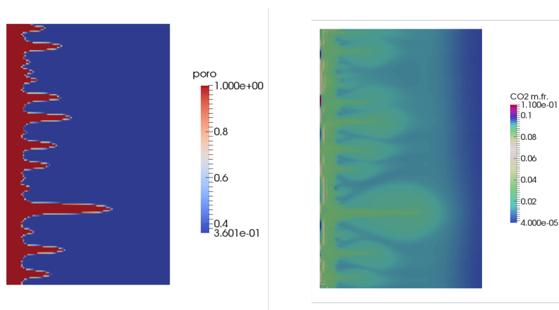
Figure 11 Smearing and retardation of wormholes due to \text{CO}_2 co-injection. Left: porosity field of conical wormhole. Right: \text{CO}_2 concentration around wormhole.
