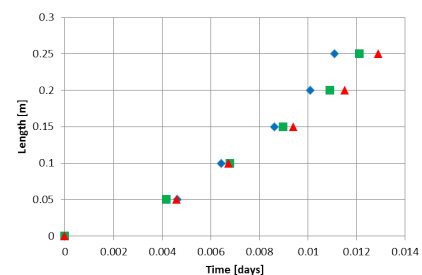
Figure 6 Wormhole dynamics for permeability perturbation at 5, 10, and 20%.
