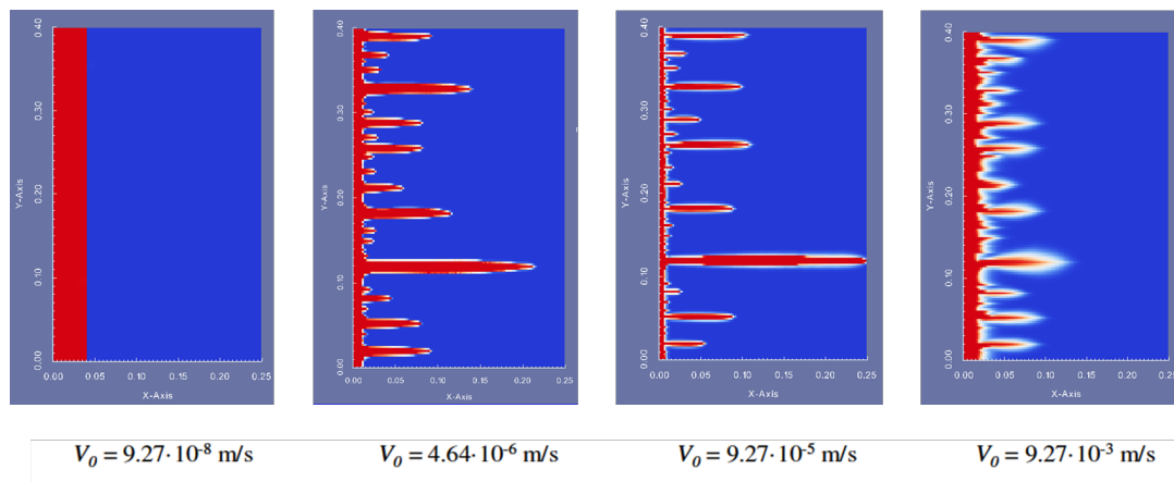
Figure 4 Wormhole dissolution patterns for increasing injection velocity in the proposed model using Darcy's assumptions with 100 \times 400 cells resolution.
