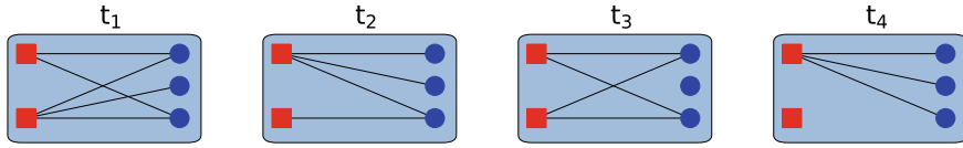
Fig. 1 Example of a temporal bipartite network at T = 4 time steps
