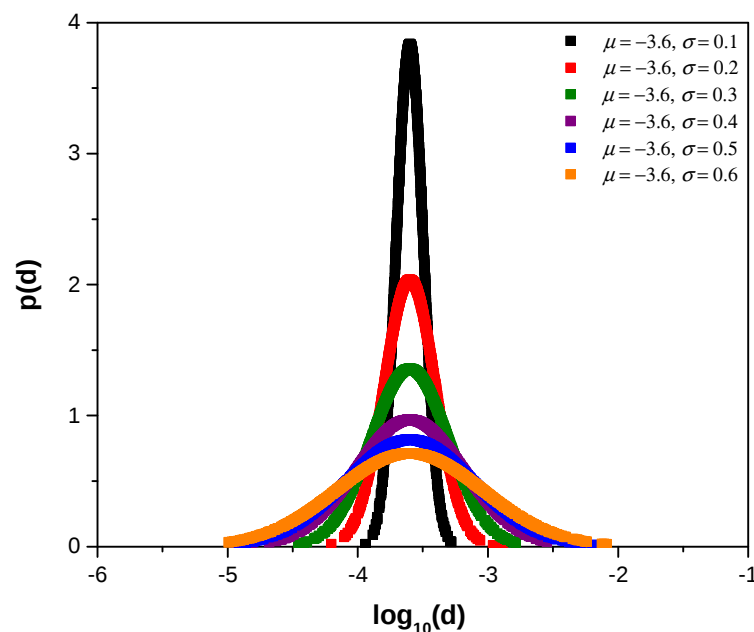
Figure 2.11 Probability density function ( p(d) ) for fracture aperture for log-normal distributions with the same mean value but different standard deviations in log-10 space.
