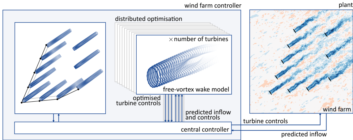
Figure 6. The finite-horizon optimisation problem for economic model-predictive control is solved in parallel with a wake model for each turbine. A central controller communicates with the wind farm to update control set points and incorporates the predicted inflow. It updates the graphs connecting upstream and downstream neighbours and distributes information. The current control framework is open loop and does not utilise wind farm measurements for state estimation or parameter updates.
