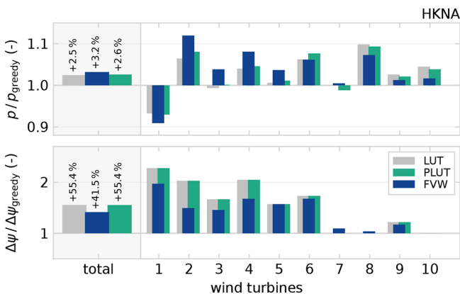
Figure 13. The FVW controller improves power production with respect to the LUT and PLUT approaches and reduces the increase in total yaw actuation required. The gain comes mostly from turbines 2 to 7, whereas turbines 1 and 8 to 10 lose some power with respect to the LUT and PLUT controllers.
