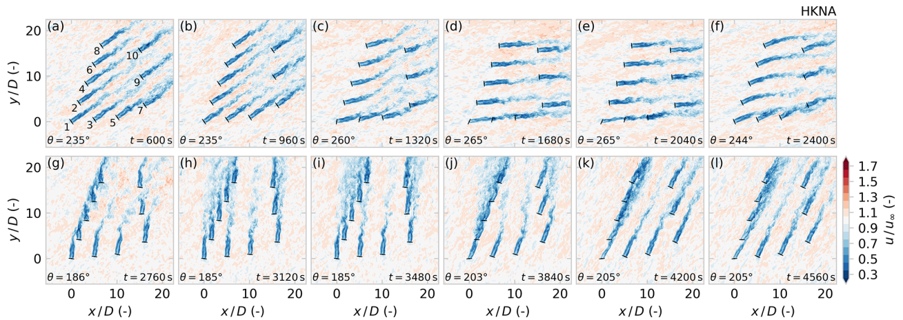
Figure 12. Series of hub height flow snapshots from LES of the HKNA test case with the FVW controller. In the initial transient, (a) all wind turbines are aligned with the mean inflow direction. Wake steering solutions are illustrated in (d) and (e) for the southern row of wind turbines 1, 3, and 5 and (k) and (l) for the western row of wind turbines 1, 2, 4, 6, and 8. Waked turbines have a reduced yaw offset because of the modelling of secondary steering effects. For certain wind directions, long wakes impact farm performance, which are not accounted for in the FVW due to the limited prediction horizon. For example, (d) and (e) show the wake of turbine 4 impinging on turbine 9 and (h) and (i) show turbine 8 operating in the wake of turbine 3.
