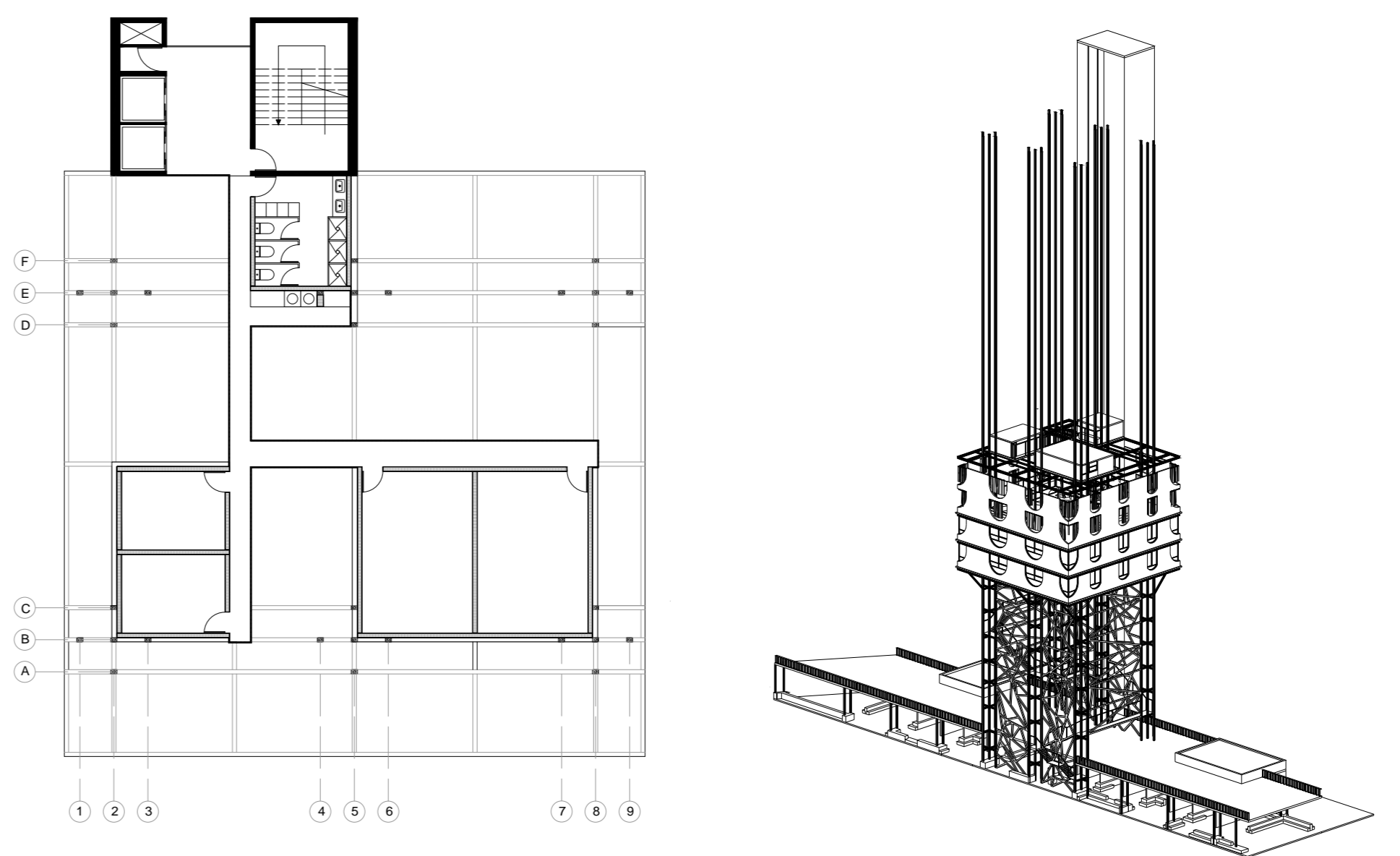
FLOOR PLAN +46.00 1:250
