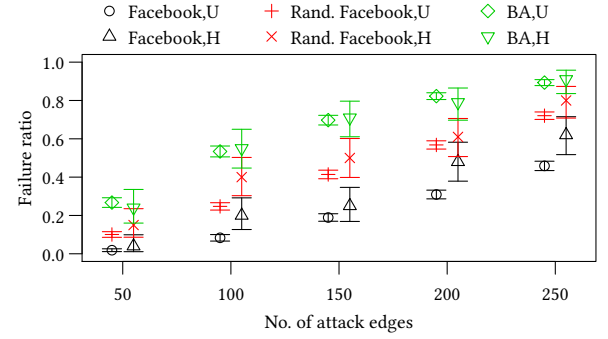
Figure 7: Obtained mean failure ratios for the Facebook graph, its randomized version and the BA graph, for a varying number of attack edges and uniformly (U) as well as highest-degree (H) victims. The bars below and above each mean value represent 95% confidence intervals.
