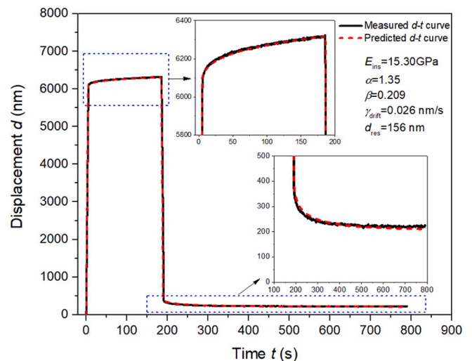
Fig. 9. A typical comparison between the measured and predicted displacement-time curve for one w/c 0.4 sample from test series 5.
